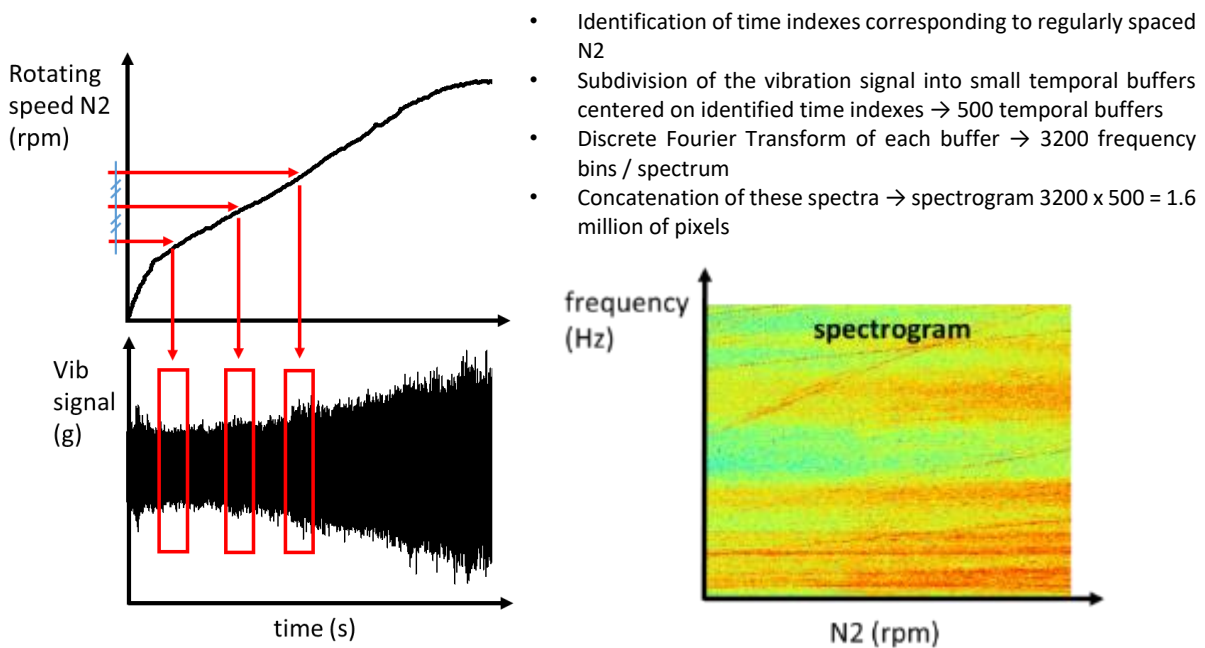
Figure 2: Diagram explaining how spectrograms are calculated and plotted based on the engine speed (N2)
