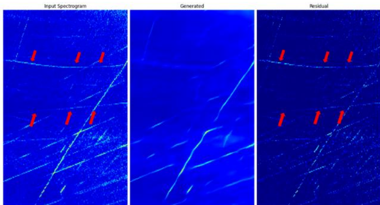
Figure 10: Zoom on spectrogram3 around the red arrows.
