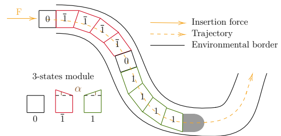
Fig. 1. Principle of the 3-states module based snake-like robot developed to perform complex trajectories in confined environment. Each state of the module is identified as a balanced ternary signed-digit, i.e. \bar{1} , 0, 1.
