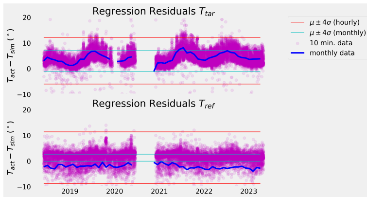
Figure 4: Random Forest Regression residuals analysis for gear bearing 1.
