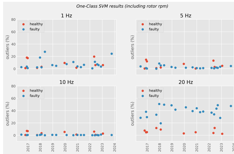
Figure 6: One-Class SVM results with rotor rpm.
