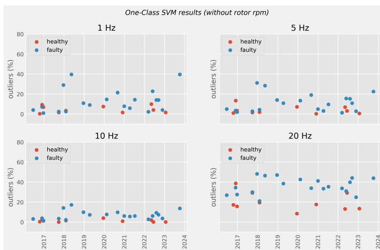
Figure 5: One-Class SVM results without rotor rpm.
