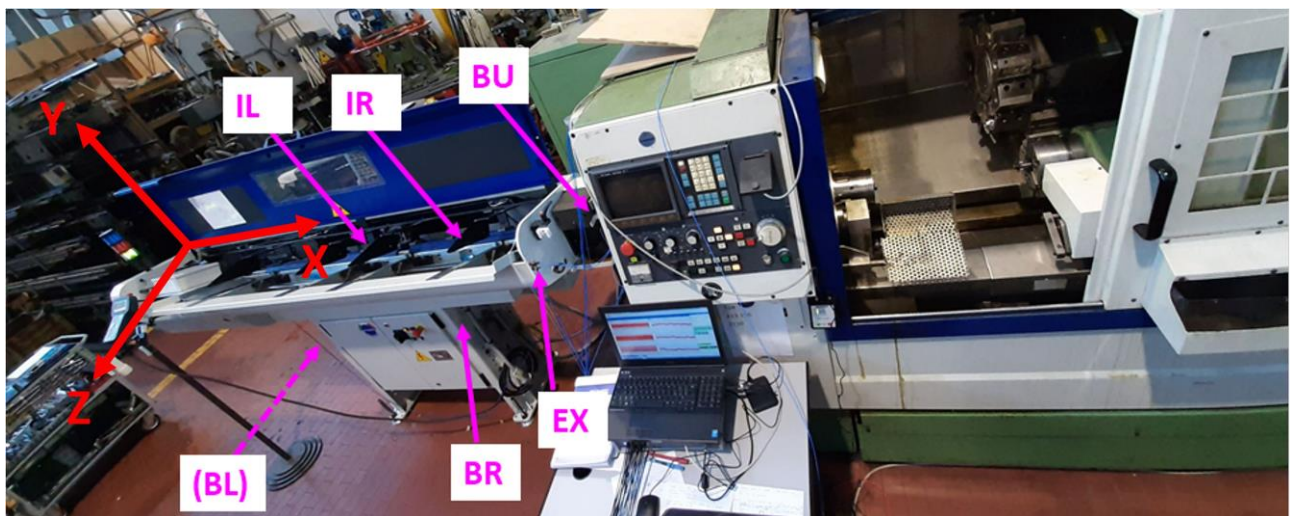
Figure 3: test setup.
