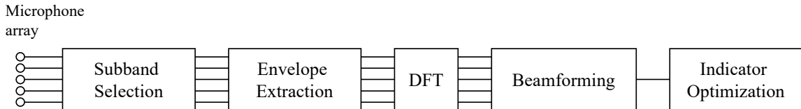
Figure 2: Proposed Methodology.
