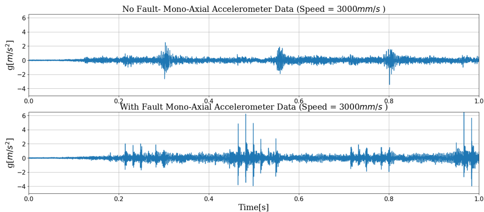
Figure 7: Vibration Data Acquired at the Mover Speed of 3000 mm/s
