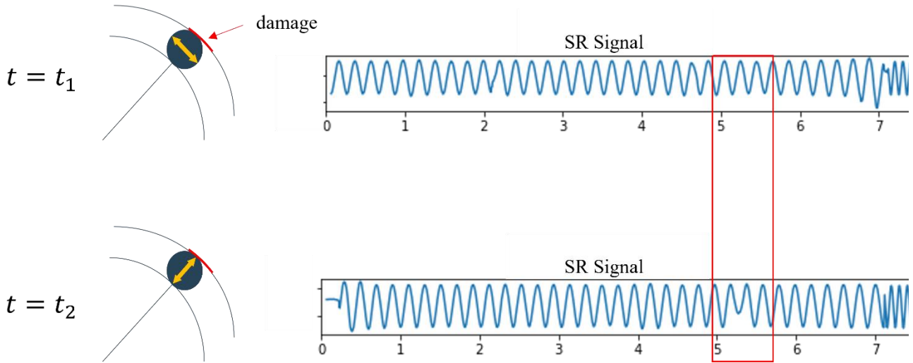
Figure 2: The measurement orientation of the SR relative to the surface damage can significantly influence the resulting calculated load signal, causing it to vary depending on the position of the sensor.
