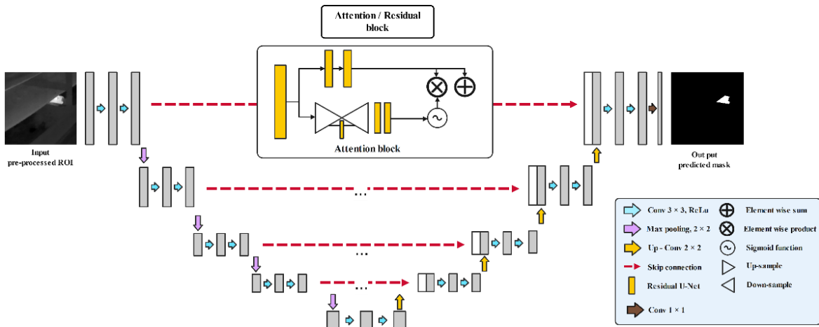
Figure 1: AResU-Net architecture
