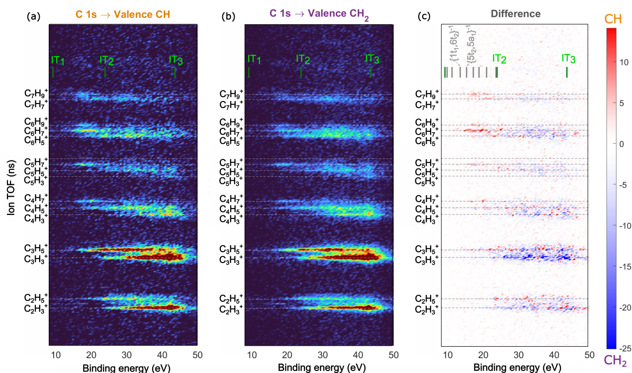
Figure 4. AEPICO map of ions and Auger electrons detected in coincidence for the CH (a) and CH_2 (b) resonant excitations at 287.1 eV and 287.6 eV, respectively. The difference between the AEPICO maps (a,b) is shown in (c), the intensity in red indicates ions which had higher yield in (a) i.e., the CH site excitation and the intensity in blue indicates ions which had higher yield in (b) i.e., the CH_2 site excitation. The first, second and third ionization thresholds are labeled as (IT 1 ), (IT 2 ) and (IT 3 ), respectively. The maps (a,b) are area normalized.
