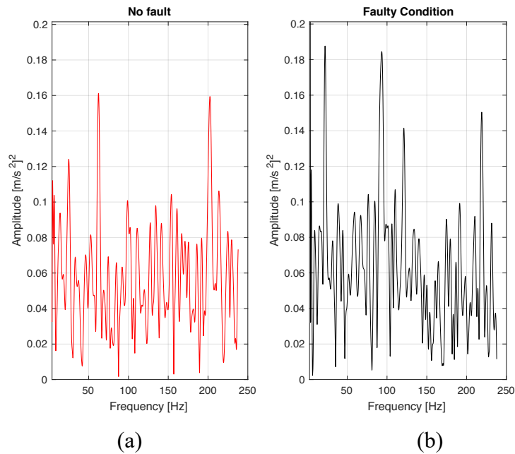
Fig. 4 Squared envelope of gear vibration signal with a SNR of 3 dB a) non-faulty condition, b) faulty condition
