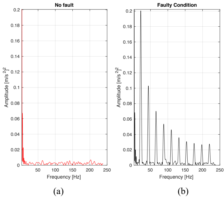
Fig. 3 Squared envelope of gear vibration signal with a SNR of 30 dB a) non-faulty condition, b) faulty condition
