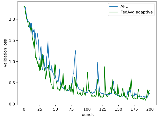
(b) Global validation loss
