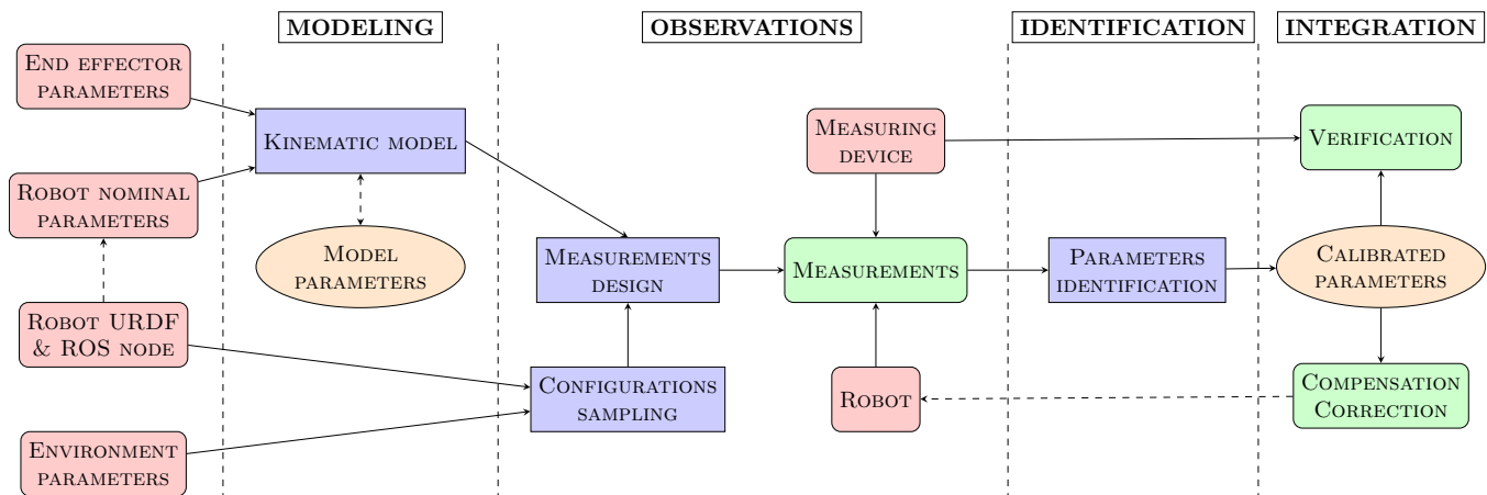
Fig. 1: Description of the overall kinematic calibration procedure
