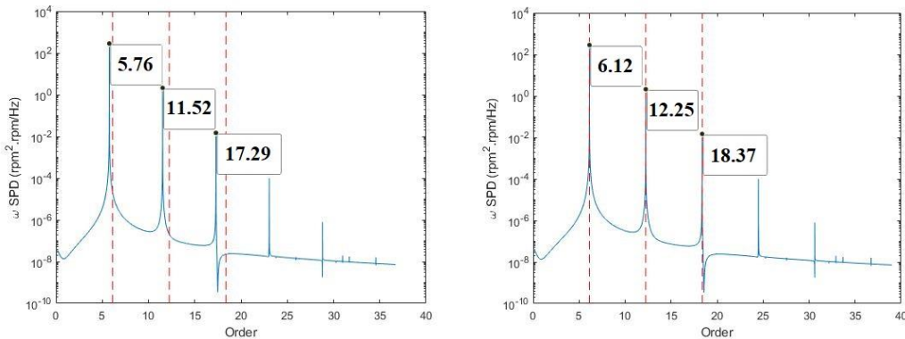
Figure 2: order spectrum for a cyclic excitation of 10% Cm at 6.126 events per revolution. Orders are based on angle-averaged velocity (left) and time-averaged velocity (right).
