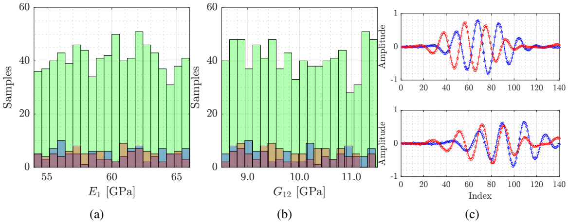
Figure 4: Surrogate model evaluation. (a) E_1 Histogram for training (■), validation (■) and test (■); (b) G_{12} Histogram; and (c) Comparison between surrogate model (○) and FE model (—) for different values of test data
