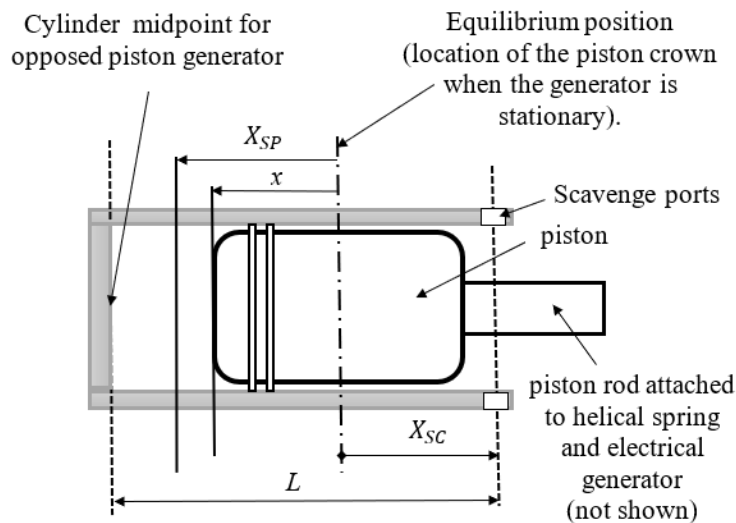
Figure 1b: Free-piston generator position variables.
