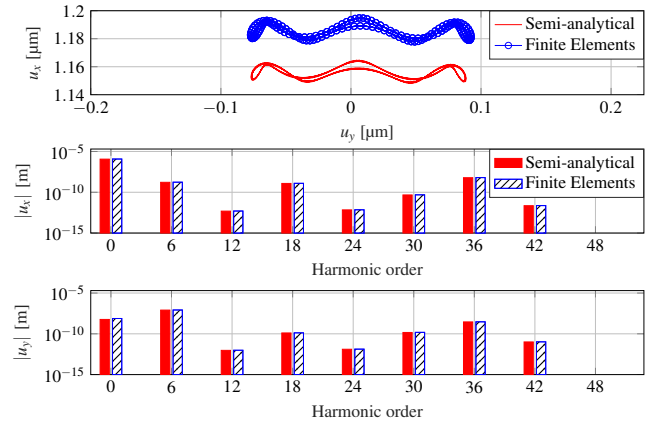
(b) Displacement of the center of the shaft over time at 2000 rpm, and Fourier transformation of u_x and u_y using the semi-analytical and finite element models
