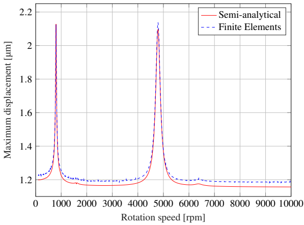
(a) Maximum displacement during one cycle on the shaft, solved by mode superposition in weak coupling using the finite element model (100 nodes) and the semi-analytical model (40 modes)
