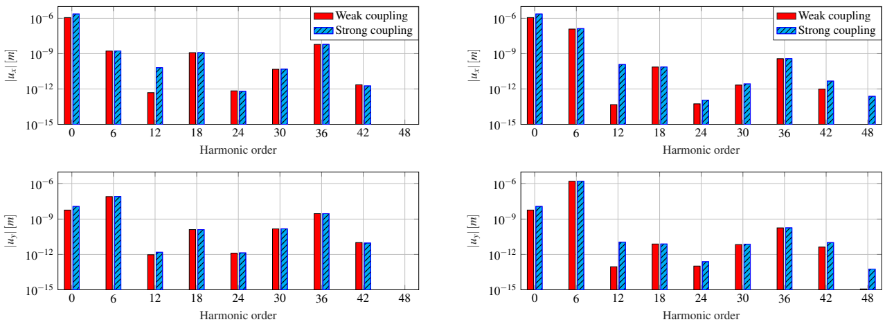
(a) Harmonic content of displacements u_x and u_y at 2000 rpm
