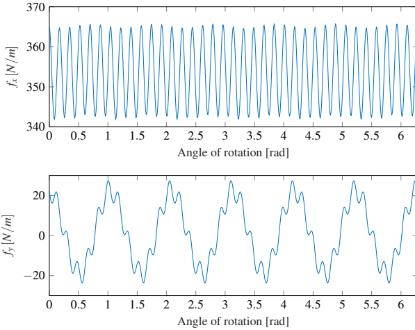
(a) Linear magnetic forces f_x(x_0, y_0) and f_y(x_0, y_0) with a static eccentricity \varepsilon_s of 10% of the air gap along the x axis as a function of the rotation angle
