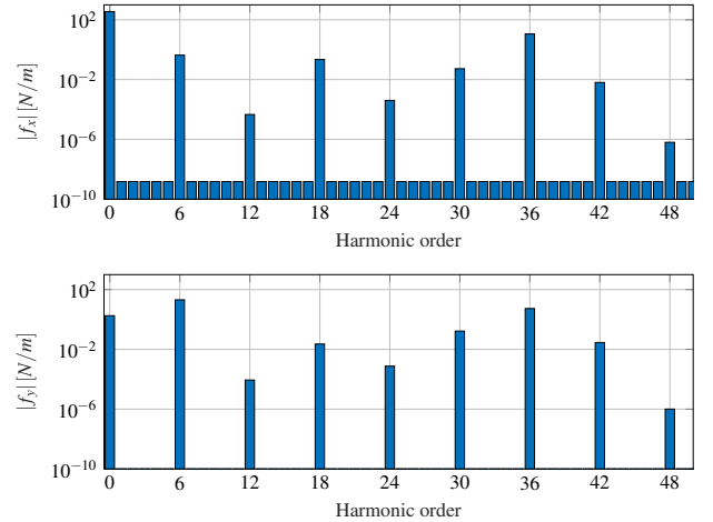
(b) Amplitude spectrum of the linear forces f_x(x_0, y_0) and f_y(x_0, y_0) , forces generated by a machine with 3 pairs of poles and 36 slots
