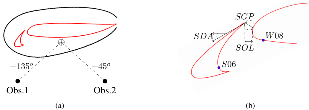
Figure 1: a) Geometry of the two element high-lift device from the VALIANT project[1], with FWLH surface and relative observer positions. b) Three variable slat coordinate system relative to the airfoil and two wall pressure probes S06 and W08.
