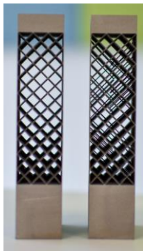
Figure 3 : Manufactured demonstrator (left without resonator ; right with resonators)
