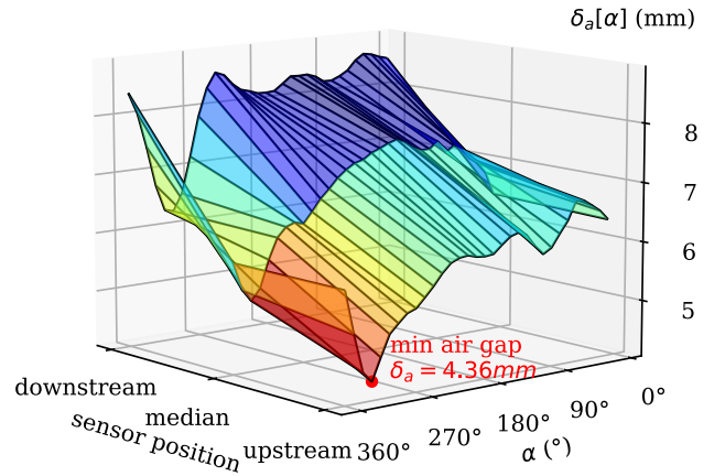
(b) Unfolded 3d air gap profile allowing to capture the general trends in stator deformation.
