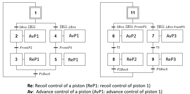
(b) PLC Logic for the Use Case (SFC)
