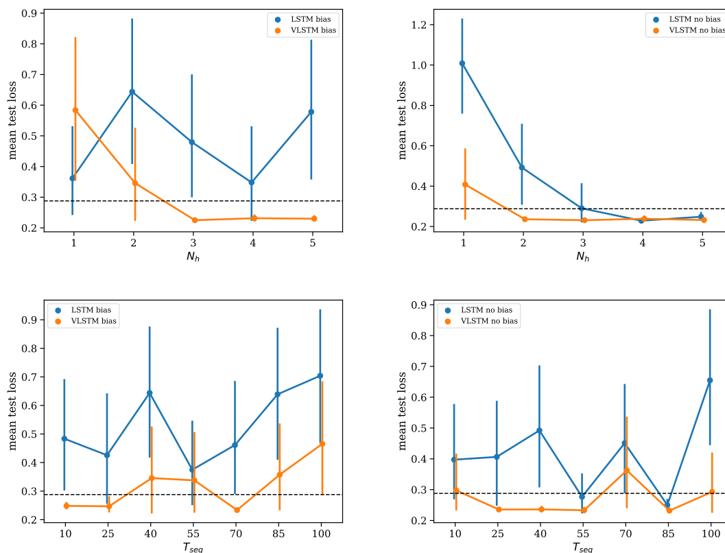
Figure 2: Volatility prediction. Upper plots: mean test loss vs the memory cell dimension N_h ( T_{seq} = 40 ); lower plots: mean test loss vs the sequence length T_{seq} ( N_h = 2 ). Left plots: (V)LSTMs with bias weights; right plots: (V)LSTMs with no bias weights. The dashed line is the average MSE of predictions made with rough volatility models.
