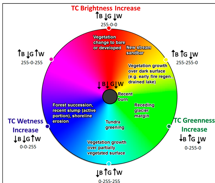
Figure G1. Color map legend for Tasseled Cap trend visual interpretation produced by Fraser et al. (2014).
