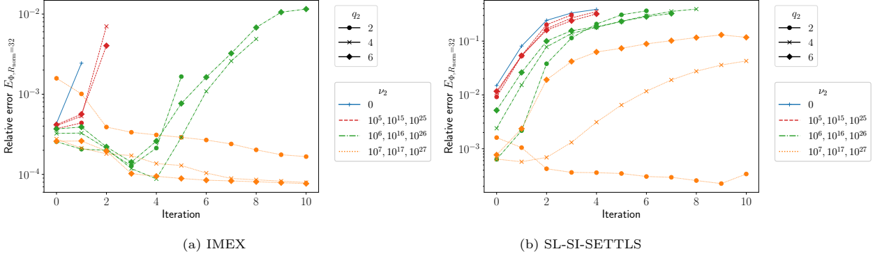
Figure 12: Gaussian bumps test case: relative error E_{\Phi, R_{\text{norm}}=32} between the PinT and fine solutions at t = T along iterations for R_{\text{norm}} = 32 , with IMEX (left) or SL-SI-SETTLS (right) being used as a coarse time-stepping scheme, as a function of the viscosity coefficients applied on the coarsest level. All simulations use configuration (N_{\text{levels}}, m_c, N_{\text{relax}}, M_{\text{coarse}}) = (3, 2, 0, 128) . No viscosity is applied on the finest and intermediate levels. Viscosity coefficients expressed in \text{m}^q \text{s}^{-1} .
