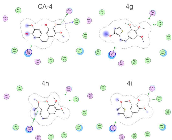
Fig. 7. Top docking pose obtained for CA-4, (Z)-4g, (Z)-4h and (Z)-4i. Docking pose with (Z)-4h shows a cation- \pi interaction between its thiophene motif and K352 of the \beta monomer. Hydrophobic interactions are not represented.
