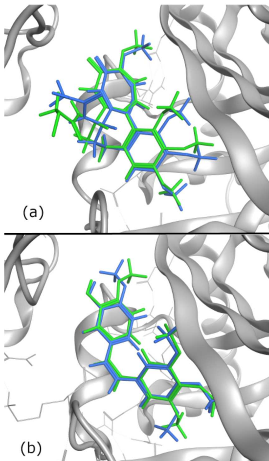
Fig. 5. (a) Comparison of top docking pose (green) and crystal pose (blue) of the colchicine analog CN2 (2-mercapto-n-[1,2,3,10-tetramethoxy-9-oxo-5,6,7,9-tetrahydro-benzo[a]heptalen-7-yl]acetamide). (b) Comparison of top docking pose (green) and crystal pose (blue) of CA-4
