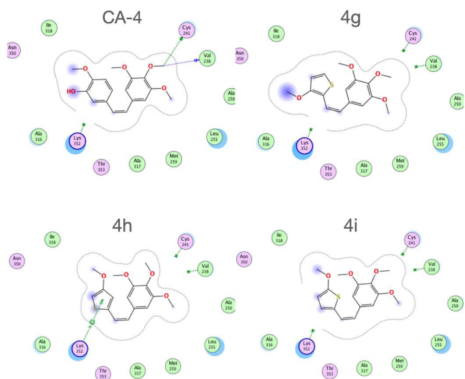
Fig. 7. Top docking pose obtained for CA-4, (Z)- 4g , (Z)- 4h and (Z)- 4i . Docking pose with (Z)- 4h shows a cation- \pi interaction between its thiophene motif and K352 of the \beta monomer. Hydrophobic interactions are not represented.
