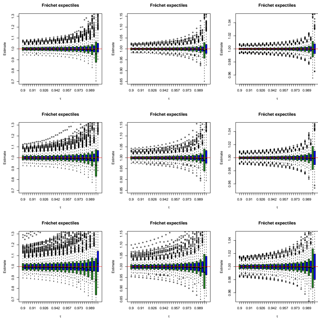
Figure 6: Example of the Fréchet distribution. Boxplots of \hat{\xi}_{\tau,n} (green) and \check{\xi}_{\tau,n} (blue), normalized by the true value \xi_{\tau} calculated through the Newton-Raphson algorithm, for a regular grid of 20 values of \tau \in [0.9, 0.995] . We take 1,000 Monte-Carlo replications of an independent sample of size n = 1,000 (left), 10,000 (middle) and 100,000 (right), where \gamma = 1/5 (top panels), 1/4 (middle panels) and 1/3 (bottom panels).
