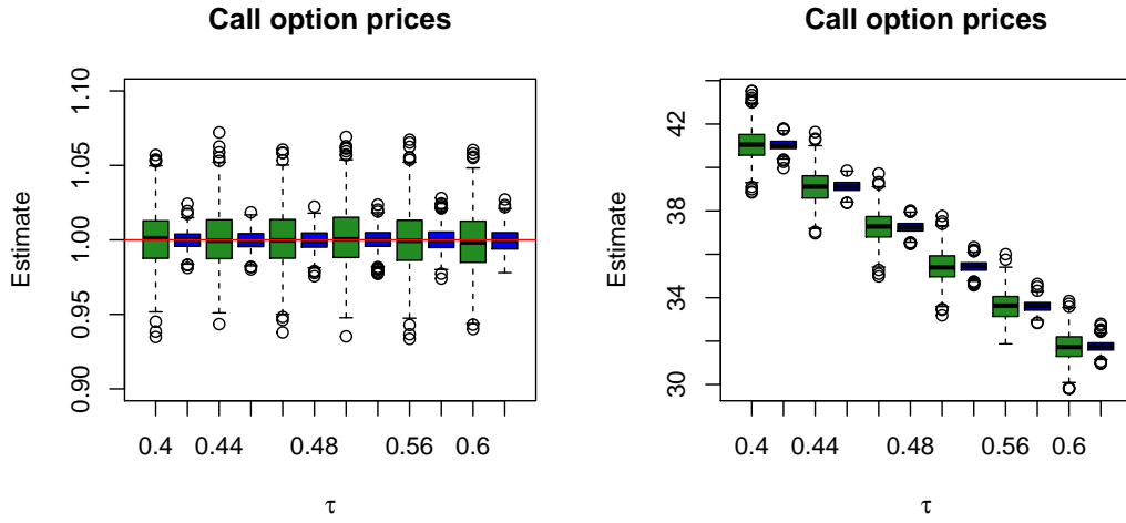
Figure 5: Option pricing example. Left panel: Boxplots of \widehat{C}_0^{(BS)}(\xi_\tau)/C_0^{(BS)}(\xi_\tau) (green) and \widetilde{C}_0^{(BS)}(\xi_\tau)/C_0^{(BS)}(\xi_\tau) (blue), in the Black-Scholes model with volatility \sigma^2 = 1 . Right panel: Boxplots of \widehat{C}_0(\xi_\tau) (green) and \widetilde{C}_0(\xi_\tau) (blue), in the Heston model with \kappa = 2 , \theta = 0.8 , \nu_0 = 1 , \sigma^2 = 0.01 and \rho = 0.5 . In both examples, the time horizon is T = 1 , the risk-free interest rate is r = 5\% = 0.05 and the initial condition is S_0 = 100 . We consider the values \tau = 0.4, 0.44, 0.48, 0.52, 0.56, 0.6 , and use 1,000 Monte-Carlo replications of an independent sample of size n = 10,000 from S_T .
