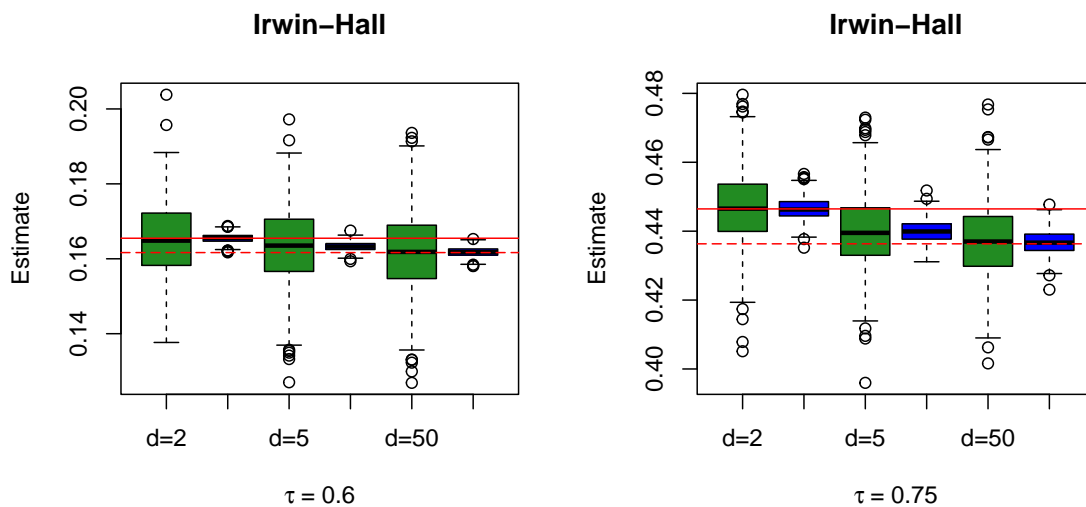
Figure 2: Example of the Irwin-Hall distribution. Boxplots of (\tilde{\xi}_{\tau,n}^{(d)} - d/2)/\sqrt{d/12} (green) and (\tilde{\xi}_{\tau,n}^{(d)} - d/2)/\sqrt{d/12} (blue) for \tau = 0.6 (left) and \tau = 0.75 (right). In both panels, we take, from left to right, d \in \{2, 5, 50\} , and use 1,000 Monte-Carlo replications of an independent sample of size n = 10,000 . The full red line is (\xi_\tau(\text{T}) - 1)/\sqrt{1/6} , where \xi_\tau(\text{T}) is the expectile of the triangular distribution (known in closed form), and the dashed red line is the expectile \xi_\tau(\text{G}) of the standard Gaussian distribution (approximated via the Newton-Raphson algorithm).
