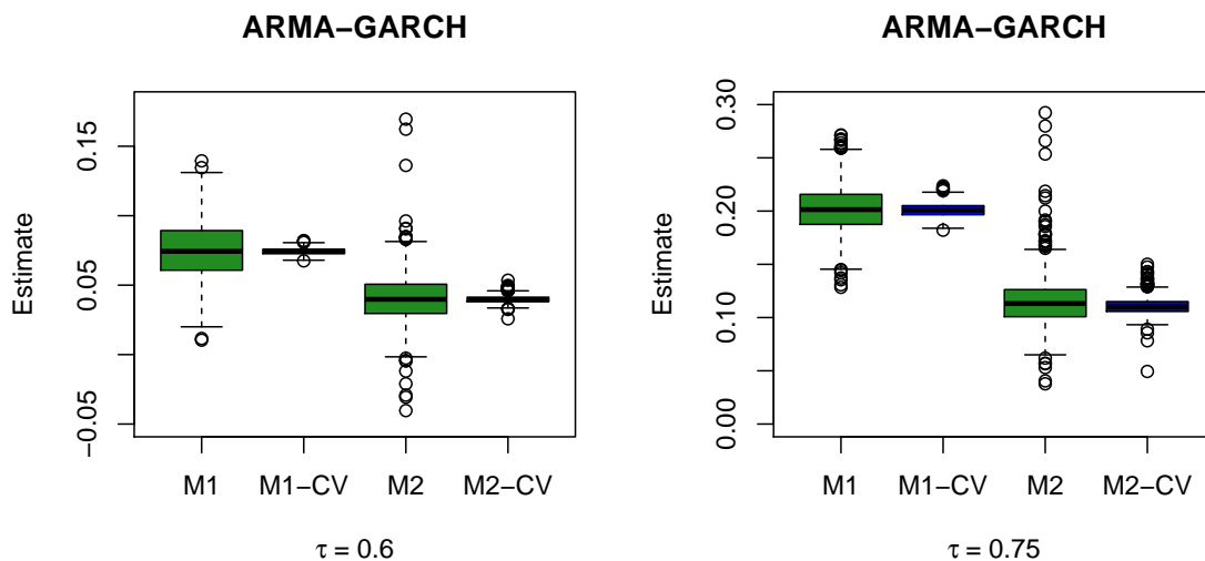
Figure 3: Example of the ARMA(1,1)-GARCH(1,1) process. Boxplots of \hat{\xi}_{\tau,n} (green) and \tilde{\xi}_{\tau,n} (blue) for \tau = 0.6 (left) and \tau = 0.75 (right). In model 1 we let (\alpha, \beta) = (0.1, 0.85) and in model 2 we let (\alpha, \beta) = (0.85, 0.1) . Both models have \phi = 0.9 , \theta = 0.5 , \omega = 0.001 , and the \varepsilon_t are standard Gaussian innovations. In each setting, 1,000 Monte-Carlo replications of an independent sample of size n = 10,000 were used.
