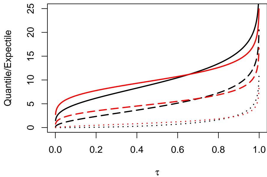
Figure C.4: Quantiles (black) and expectiles (red) of the chi-squared distribution with 1 (dotted curves), 5 (dashed curves) and 10 (solid curves) degrees of freedom, as functions of \tau \in (0, 1) .
