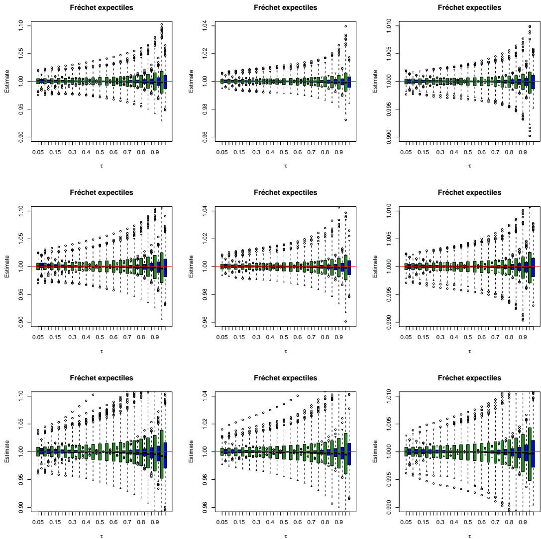
Figure 1: Example of the Fréchet distribution. Boxplots of \hat{\xi}_{\tau,n} (green) and \tilde{\xi}_{\tau,n} (blue), normalized by the true value \xi_{\tau} calculated through the Newton-Raphson algorithm, for \tau \in \{0.05, 0.10, \dots, 0.95\} . We take 1,000 Monte-Carlo replications of an independent sample of size n = 1,000 (left), 10,000 (middle) and 100,000 (right), where \gamma = 1/5 (top panels), 1/4 (middle panels) and 1/3 (bottom panels).
