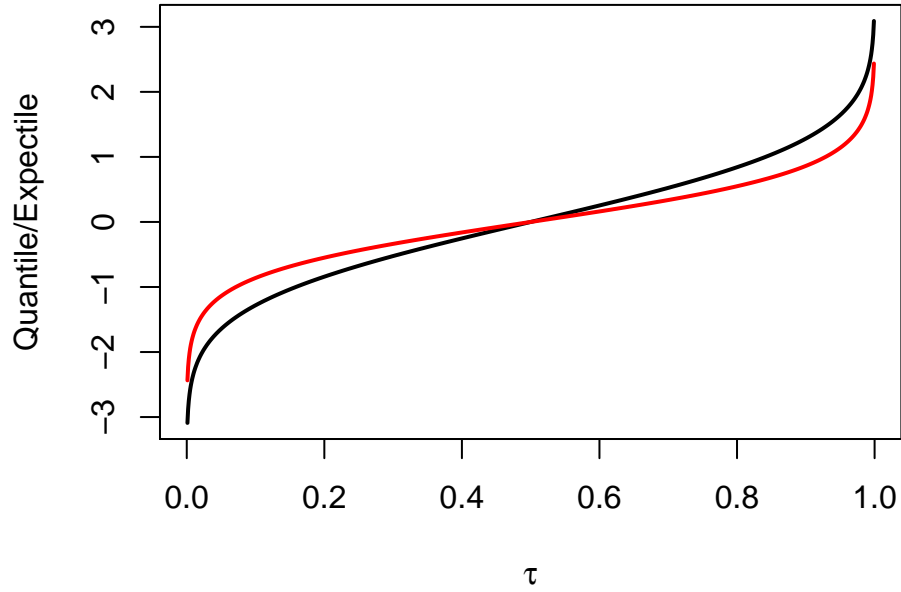
Figure C.1: Quantiles (black) and expectiles (red) of the standard Gaussian distribution, as functions of \tau \in (0, 1) .
