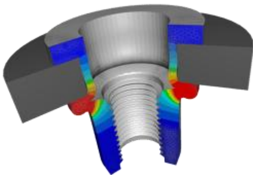
Figure 1 : Mechanical joining
