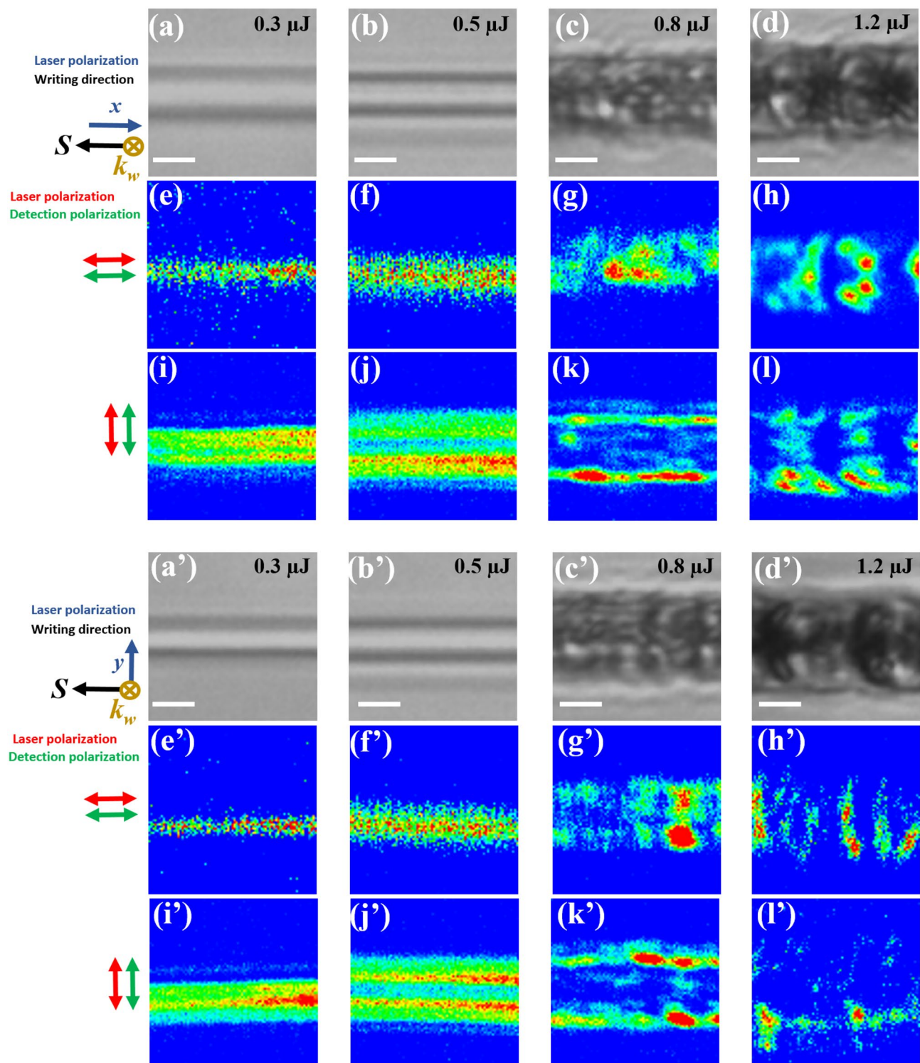
Figure 5. Optical microscopy images of laser tracks by the femtosecond laser pulses with pulse energies of 0.3 \mu\text{J} ( a, a' ) or 0.5 \mu\text{J} ( b, b' ) or 0.8 \mu\text{J} ( c, c' ) or 1.2 \mu\text{J} ( d, d' ) for each writing laser polarization; ( a, b, c, d ) correspond to Xx configuration and ( a', b', c', d' ) to Xy configuration in the 8%ZnO-BGG sample. ( e, f, g, h ) represents the micro-SHG mapping I_{xx} of laser tracks ( a, b, c, d ). ( i, j, k, l ) represents the micro-SHG mapping I_{yy} of laser tracks ( a, b, c, d ). ( e', f', g', h' ) represents the micro-SHG mapping I_{xx} of laser tracks ( a', b', c', d' ). ( i', j', k', l' ) represents the micro-SHG mapping I_{yy} of laser tracks ( a', b', c', d' ). Symbol of k_w indicates the laser propagation direction and S the writing direction. Scale bars in white color are 5 \mu\text{m} . The color code is optimized to the amplitude of the signal for better observation. The real intensity is provided later in Fig. 6.
