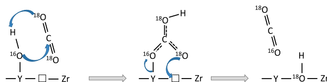
Fig. 8. Proposed oxygen exchange mechanism via hydrogen carbonate species between gas-phase \text{CO}_2 and lattice O of YSZ. Note that the \text{O--H} group may be linked to the Zr instead of the Y element.
