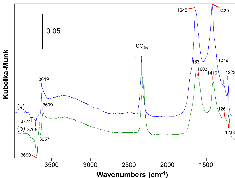
Fig. 6. DRIFT spectra collected at RT after adsorption of 4 mbar (a) C^{16}O_2 and (b) C^{18}O_2 on YSZ. These spectra were obtained after subtracting the spectra collected before CO_2 adsorption on the degassed YSZ sample.
