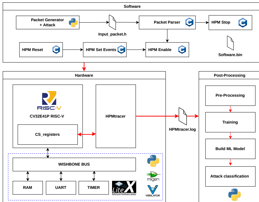
Figure 1: Testbed with tracing metrics from RISC-V CV32E41P
