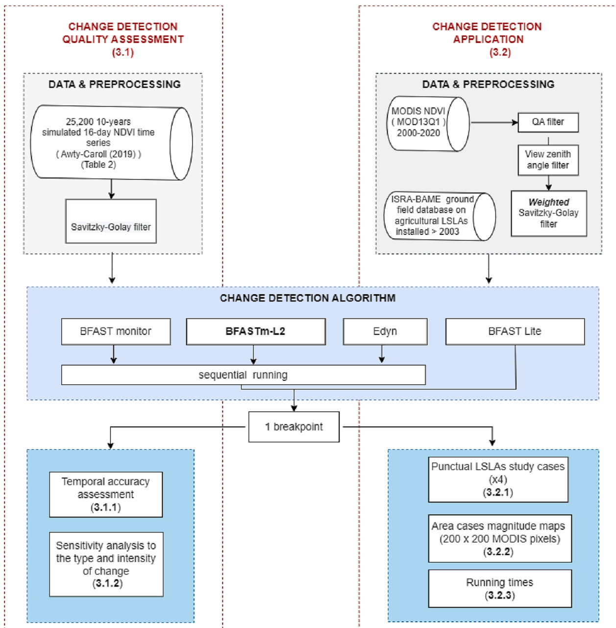
Fig. 1. Flowchart of the data and methods.
