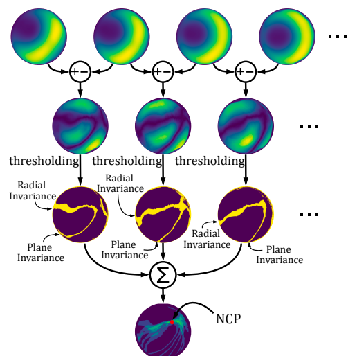
Fig. 2. SkyPole algorithm applied to experimental data for finding the NCP. Preprocessing of the first row of DoLP images consisted in filtering the images obtained using a circular averaging filter. Details of the following steps are presented in Fig. 1D.
