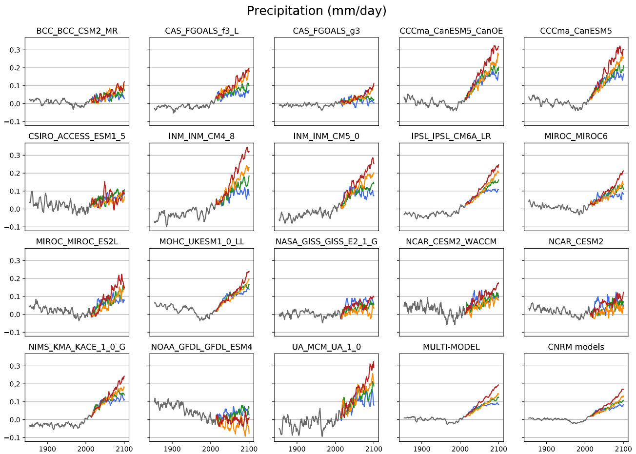
Figure 5. Times-series (1850–2100) of the 5-years running means of global land precipitation anomalies (relatively to 1985–2014) for each SSP scenario: ensemble means of the model references in Table 1 to the exclusion of the CNRM models, multi-model ensemble of these ensemble means, and ensemble mean of the CNRM models. The slope of the linear regression of each time-series is given in Figure S7 in Supporting Information S1.
