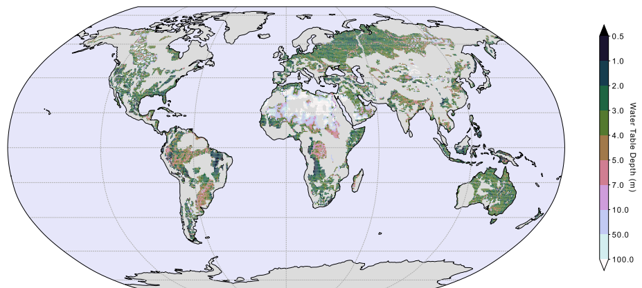
Figure 1. Global distribution of the mean water table depth simulated by the CNRM global climate models in the 218 world's major groundwater basins over the present-day period (1985–2014) in the historical experiment.
