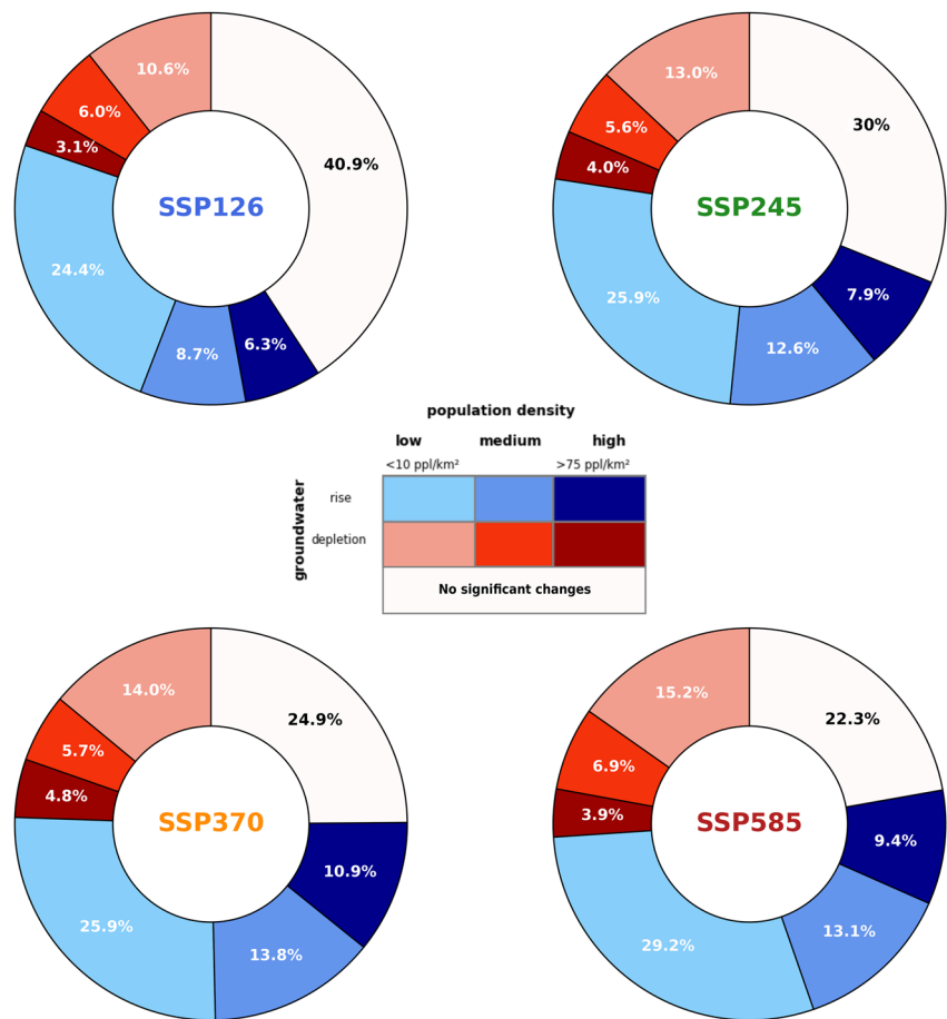
Figure 8. Share of area covered by the world's major groundwater basins where groundwater levels are projected to rise (blue) and to deplete (red). The color intensity indicates the projected population density (people per km 2 ) in 2100. The light colors correspond to areas with fewer than 10 inhabitants per square kilometer and the dark colors to areas with more than 75 inhabitants per square kilometer. The white regions correspond to areas where water table depth changes between 1985–2014 and 2071–2100 are not statistically significant.
