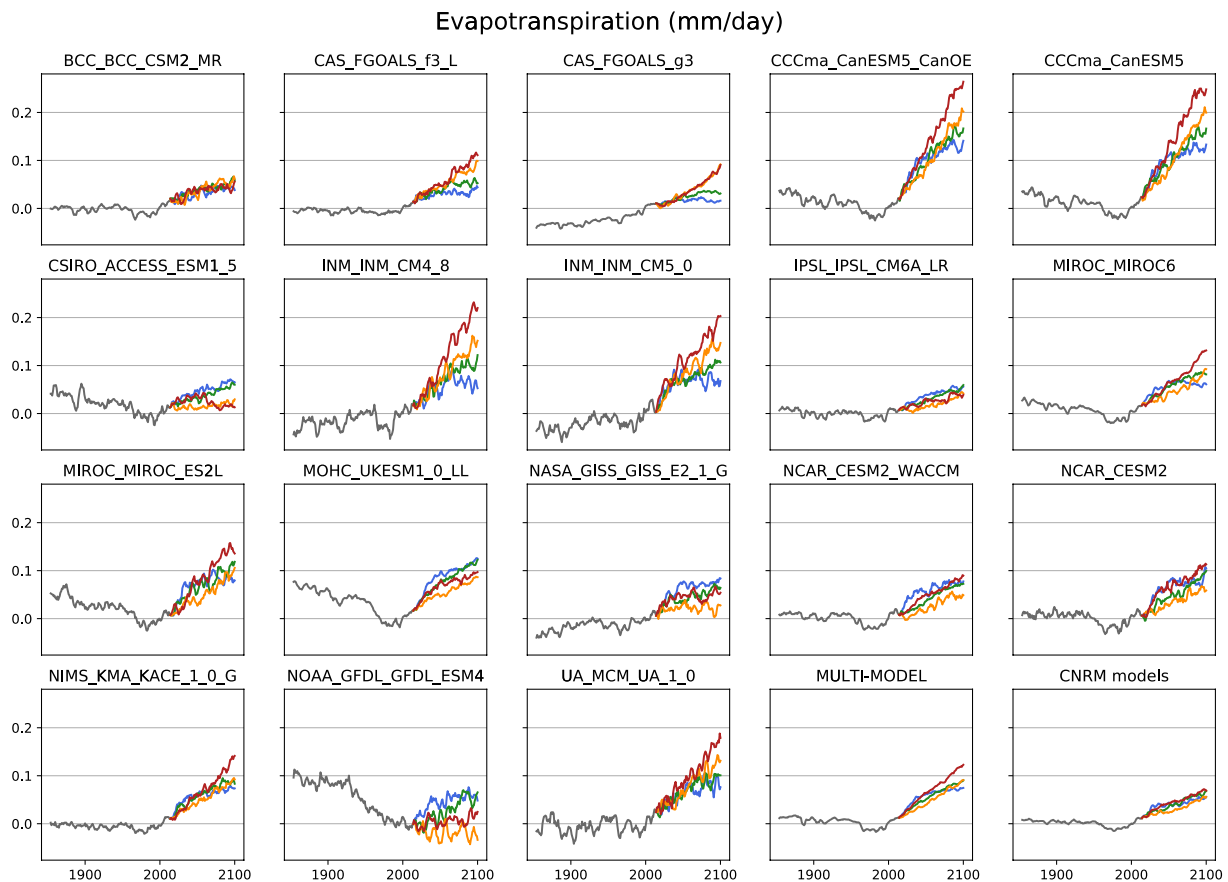
Figure 6. Same as Figure 5 but for evapotranspiration. The slope of the linear regression of each time-series is given in Figure S8 in Supporting Information S1.
