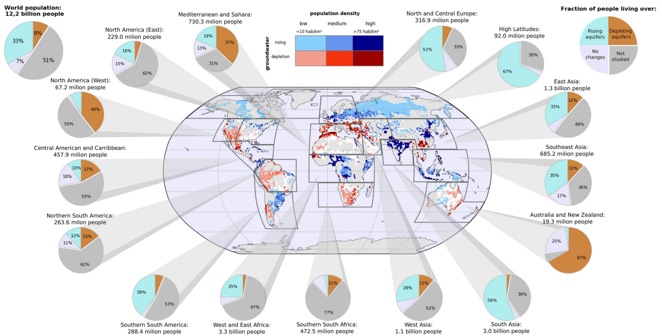
Figure 9. Evolution of water table depth and population density in 2100 with the SSP370 scenario. As in Figure 8, aquifer areas are colored blue (red) if groundwater levels are projected to rise (deepen), whilst the color intensity indicates the projected population density in 2100. The global pie chart (left hand corner) represents the distribution of the world's population which could be affected by a rising (turquoise) or a depletion (brown) of groundwater levels, or which is likely to live above an aquifer basin where future changes are not significant (white) or over unstudied areas (gray). The same pie charts are given for each selected region, defined as those used in the Atlas of Global and Regional Climate Projections in the Annex 1 of the IPCC AR5 (van Oldenborgh et al., 2013).
