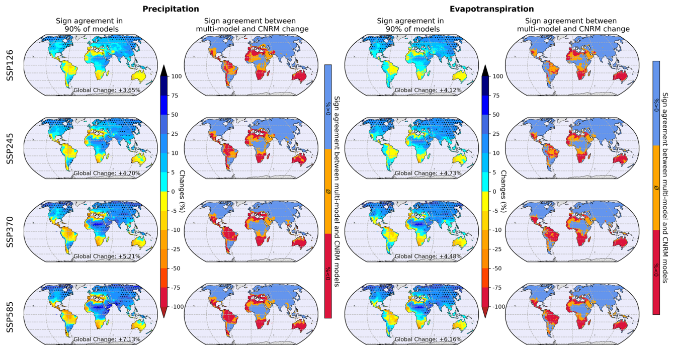
Figure 7. First column: Multi-model ensemble (excluding the CNRM models) of precipitation relative change (in %) between 1985–2014 and 2071–2100 for each SSP scenario. Black dots indicate areas where 90% of the models agree on the sign of the change. Second column: Comparison of the precipitation multi-model change with the change simulated by the CNRM models. In blue: common increase; in red: common decrease; in orange: opposite signs of change. Third and fourth columns: same as the first and second columns but for evapotranspiration.
