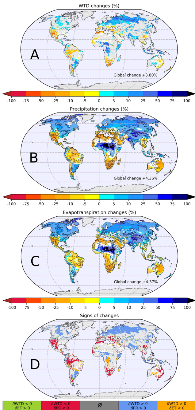
Figure 3. Water table depth (WTD) (a), precipitation (b) and evapotranspiration (c) changes (in %) between the 1985–2014 period in the historical experiment and the 2071–2100 period in the SSP370 scenario (the values of the change averaged over land are annotated on the maps). Areas in blue (red) correspond to a future WTD rise (depletion) (a) or an increase (decrease) of precipitation/evapotranspiration (b/c). The white regions correspond to areas where the changes are not statistically significant according to the FDR test (Wilks, 2006, 2016) at a 95% level of confidence. On (b) and (c), the localisation of the groundwater basins is emphasized to facilitate the comparison with WTD (a). (d) in red and blue: comparison of the sign of WTD and precipitation (PR) changes; in yellow and green: comparison of the sign of WTD and ET changes wherever the sign of precipitation changes is not consistent with the sign of WTD changes. The white regions correspond to areas where WTD changes are not statistically significant.
