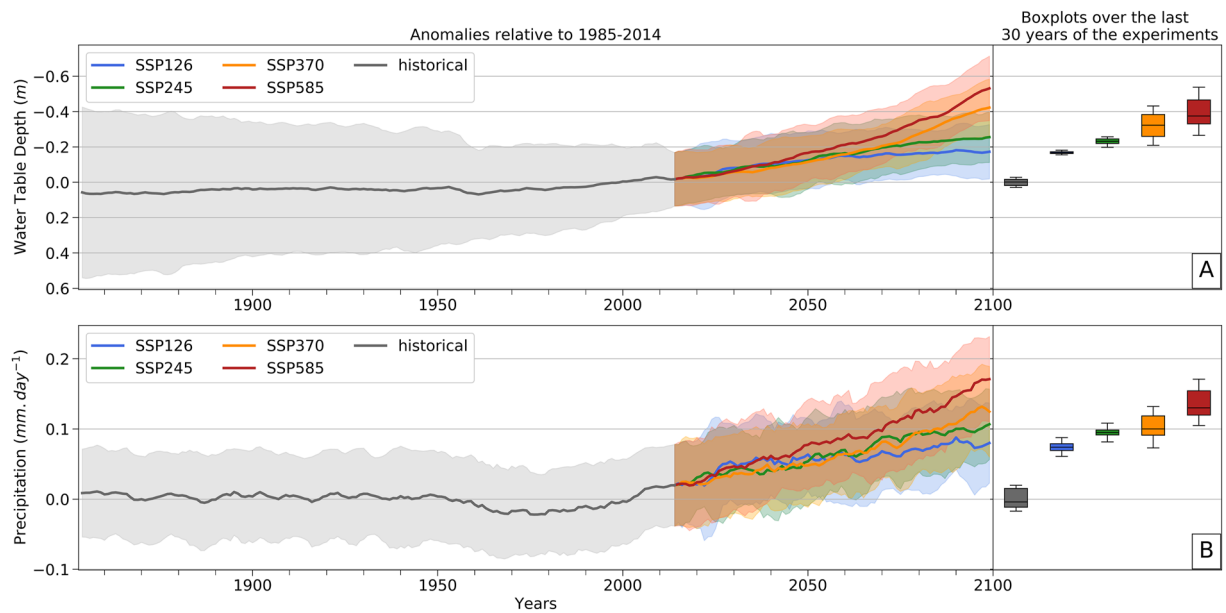
Figure 2. Time series (1850–2100) of the 5-years running average of global mean water table depth anomalies (panel (a)) and precipitation over land anomalies (panel (b)), relative to their global average in present-day climate (1985–2014 period of the historical experiment), according to all scenarios. The shading areas around the global means represent the inter-member spread ( \pm 1.64 inter-member variance) of each experiment. Boxplots further reflect the inter-member distribution of the last 30 years of the historical experiment (1885–2014) and of each scenario (2071–2100). On the boxplots, the vertical line indicates the median, the boxplot limits the first and third quartiles and the whiskers' length is 1.5 times the interquartile range.
