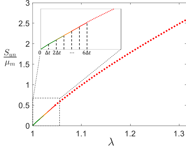
Figure 6: Macroscopic stress-stretch uniaxial responses of a microstructure with N = 64 and c = 0.4 obtained by 6 remeshing steps.
