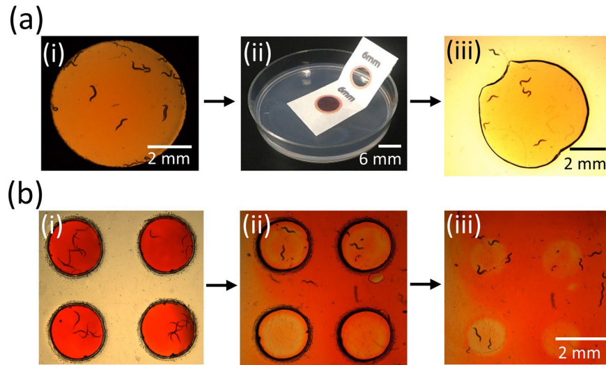
FIG. 5. Method to transfer C. elegans from paper or plastic-based 1PADs to an agar plate. The membranes are colored with a red food dye for visual ease. (a) The paper-based device having a worm population (i) is gently lowered onto the surface of the agar plate (ii). When the paper substrate is lifted upwards, its suspended agar membrane detaches and is left on the agar plate (iii). The worms are now free to migrate on the agar plate. (b) The Pluronic gel membranes containing worms (i) are lowered onto the agar plate. Once the contact is made, the suspended membranes rupture and the worms are transferred to the agar plate (ii). The plastic substrate is removed, and the worms are allowed to crawl over the agar plate (iii).
