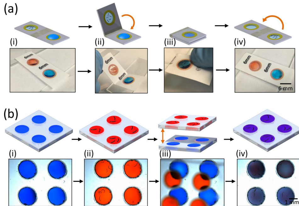
FIG. 4. Method to transfer C. elegans between two paper or plastic-based IPADs. The worm population is to be transferred from the red-colored membranes to the “target” blue-colored membranes. (a) To transfer worms between two agar membrane devices, a drop of buffer is added to the target membrane (i). The paper substrate is folded such that the red membrane having the worms is brought into contact with the target membrane [(ii) and (iii)]. After separating the two membranes, worms will transfer to the target membrane (iv). (b) To transfer worms between two plastic-based devices with Pluronic gel membranes, the top plastic-based device with red membranes (containing the worms) is aligned and lowered onto the bottom device with blue membranes [(i)–(iii)] until a physical contact is made. The top plastic device is then removed, and the worms along with some of the gel transfer to the bottom plastic device having the blue membrane (iv).
