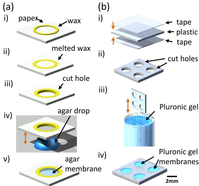
FIG. 7. Fabrication of suspended gel membranes on paper and plastic substrates. (a) Paper-based LPADs: A wax pattern is printed on chromatography paper and melted on a hot plate to create a hydrophobic barrier [(i) and (ii)]. A circular pattern is excised using a biopsy punch to create a cut hole [(iii)]. The paper is lowered onto a 100 \mu l droplet of 2% liquid agar and gently lifted, resulting in an agar membrane in the cut hole [(iv) and (v)]. Besides agar, this droplet method also works for Pluronic gel. (b) Plastic-based LPADs: A plastic sheet is taped on both sides, and multiple circular patterns are excised using an automated design cutter to create cut holes [(i) and (ii)]. The excised plastic sheet is vertically immersed into an 11.5% solution of Pluronic gel and removed, resulting in suspended membranes of Pluronic gel within the cut holes [(iii) and (iv)].
