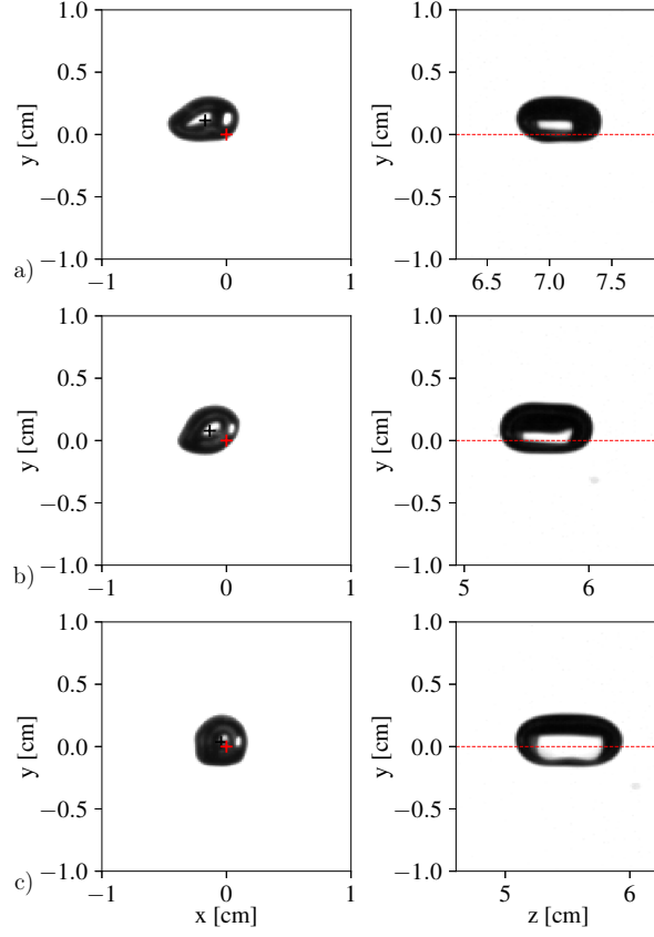
FIG. 5: Instantaneous snapshots of front view (left column) and side view (right column) of the bubble in C' solution, for V = 0.078 \text{ cm}^3 and a) \omega = 62.6 \text{ rad/s} b) \omega = 78.5 \text{ rad/s} c) \omega = 94.2 \text{ rad/s} . The red cross corresponds to the center of the tank.
