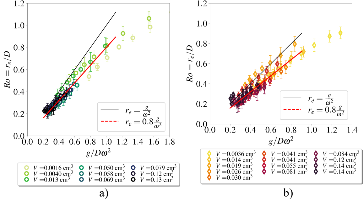
FIG. 4: Variation of the Rossby number R_o as a function of g/(D\omega^2) . a) Bubbles in C' solution. b) Bubbles in C'' solution. The black line corresponds to r_e = g/\omega^2
