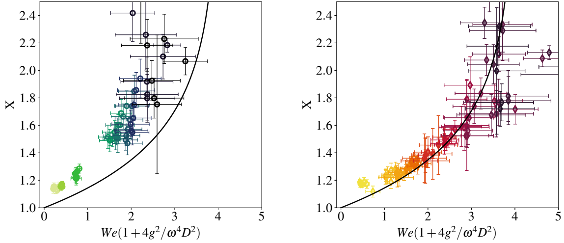
FIG. 7: Bubble aspect ratio X = L/D as a function of corrected Weber number. Left: bubbles in C' solution. Right: bubbles in C'' solution. The model works well for the C'' case, but underpredicts bubble deformation in the C' case.
