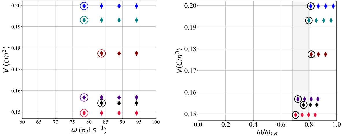
FIG. 20: Left: Volume of the bubble as a function of rotation speed: reverse break-up, i.e. break-up obtained by decreasing \omega , is observed in C'' (2 CMC) solution. Circles identify the rotation speed \omega for which rupturing occurred. Right: Volume of the broken bubble as a function of ratio \omega/\omega_{0R} .
