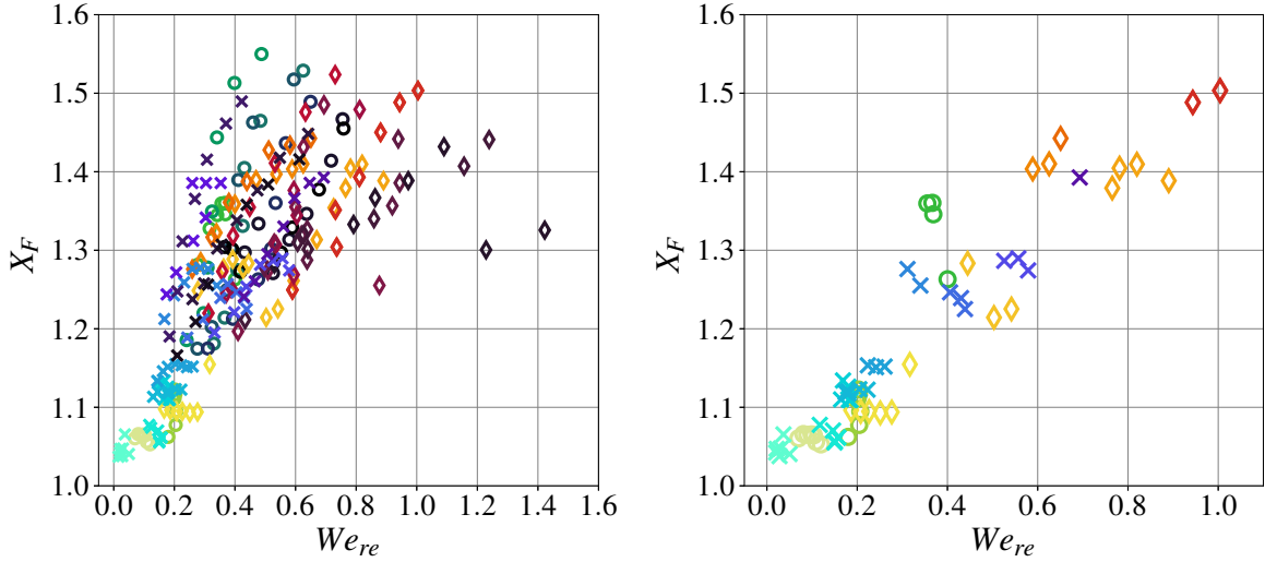
FIG. 11: Left: Front view aspect ratio X_F as a function of We_{re} . \circ : C' solution; \diamond : C'' solution; \times : demineralized water. Right: same plot, only for bubbles such that Ro > 0.5 .
