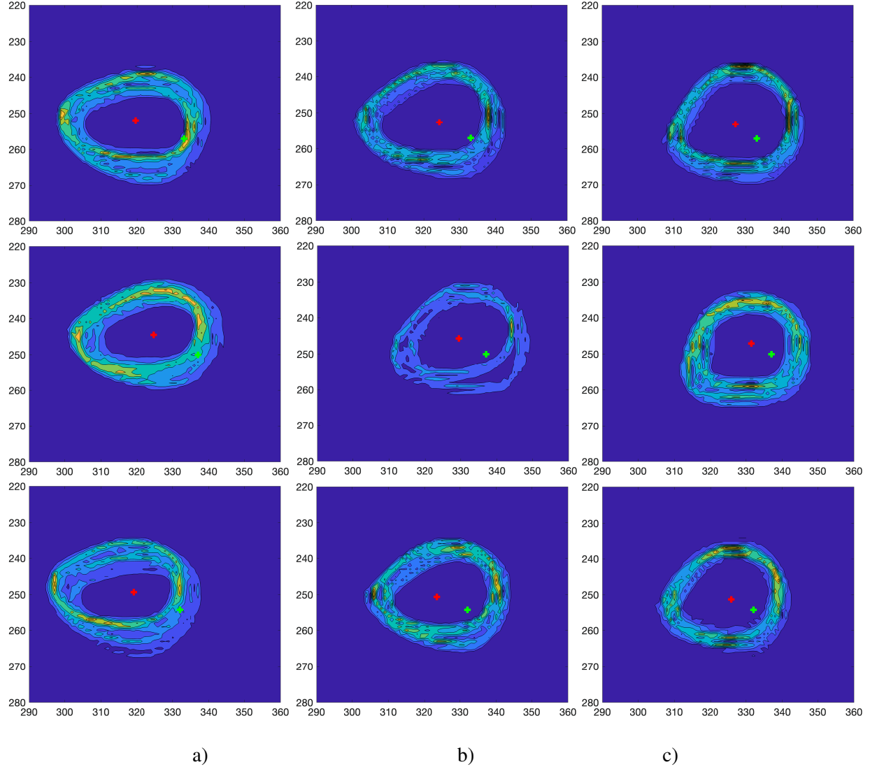
FIG. 9: Average contour of the boundary of the bubble at a) \omega = 62.6 rad/s b) \omega = 78.5 rad/s c) \omega = 94.2 rad/s; first row from top: for water solution V = 0.06 cm 3 , second row C' solution V = 0.05 cm 3 and third row C'' solution V = 0.05 cm 3 . The red cross corresponds to the associated mean position of the center of the bubble. The green cross corresponds to the center of the tank.
