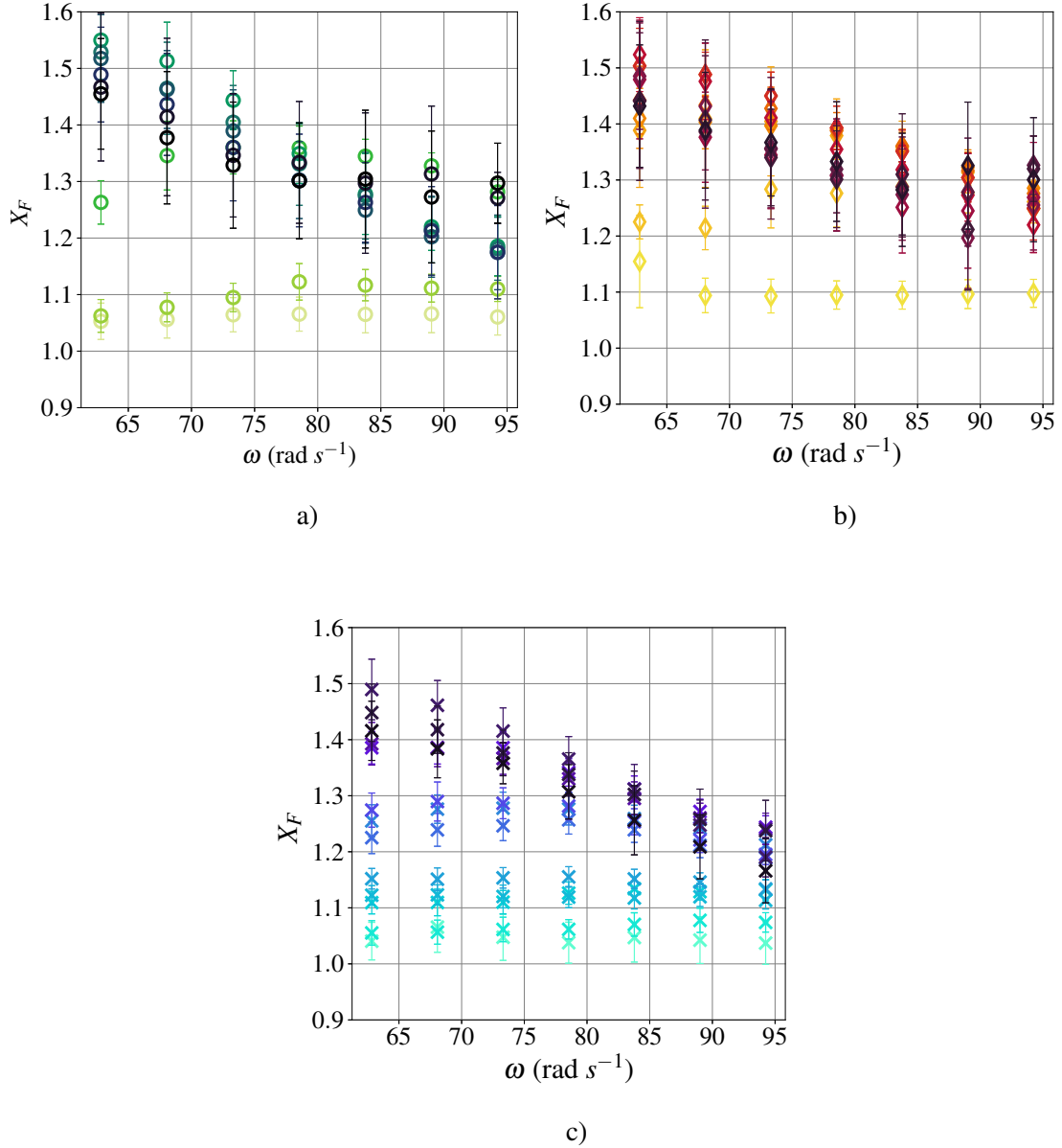
FIG. 10: Variations of the aspect ratio X_F (aspect ratio seen on front view ) as a function of the rotation speed \omega : a) bubbles in C' solution ( \circ ); b) bubbles in C'' solution ( \diamond ); c) bubbles in demineralized water ( \times ). Same caption as in figure 6.
