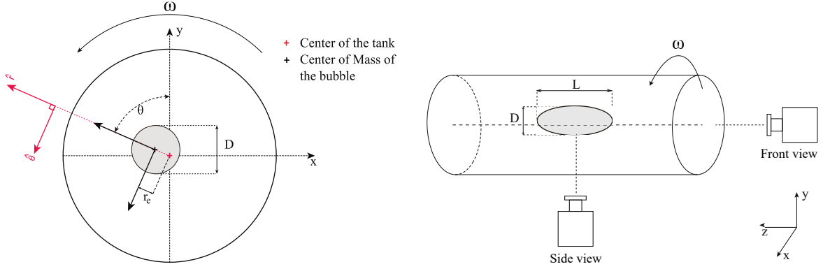
FIG. 1: Left: Configuration of the present problem, showing an approximately axisymmetric bubble close to the axis of rotation z . Right: sketch of the experimental set-up showing the positioning of the cameras relative to the rotating tank.
