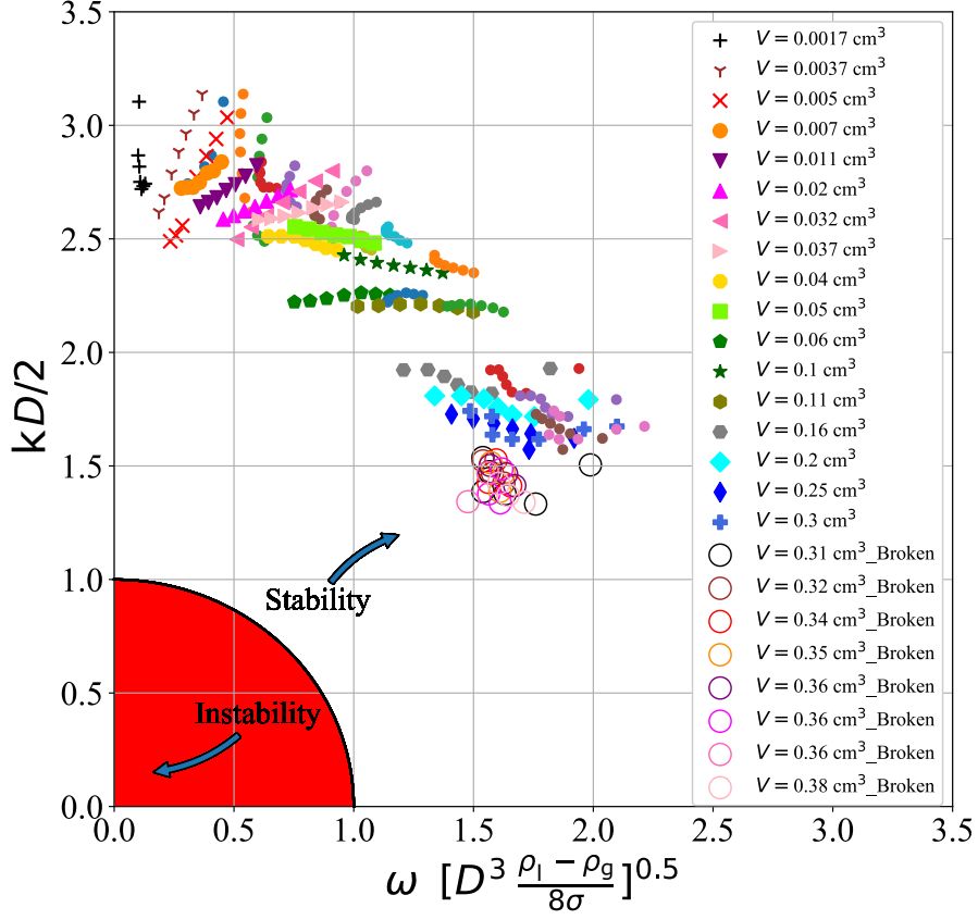
FIG. 16: Stability criterion proposed by Rosenthal [23], in the case of a bubble aligned with the axis of rotation. Here k is the wave number as 2\pi/\lambda , and \lambda is the wavelength of the considered perturbation. Experimental data points were plotted for perturbations such that \lambda = L/2 . All the experimental demineralized water data lie in the stable part of the diagram.
