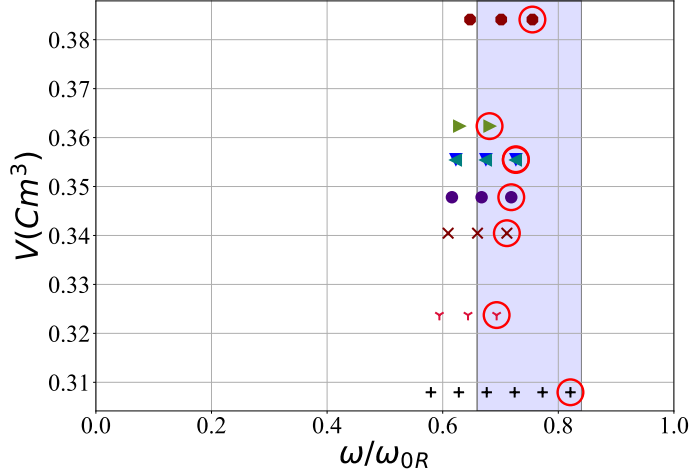
FIG. 18: Volume of the bubble as a function of ratio \omega/\omega_{0R} , ratio between tank rotation frequency, and eigenfrequency of the equivalent spherical bubble, for all experimental series experiencing break-up in water. Circles identify the conditions for which rupturing occurred.
