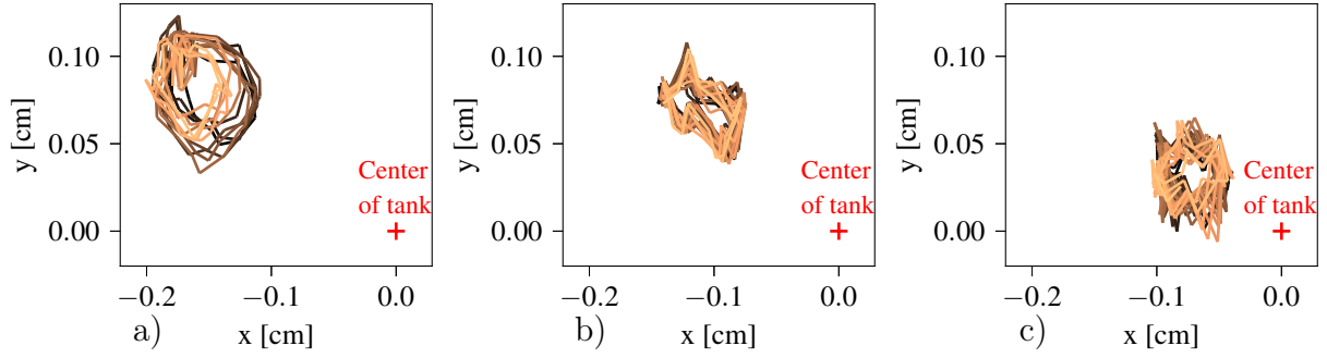
FIG. 3: Limit cycles described by bubble, for C' solution, V = 0.078 \text{ cm}^3 and a) \omega = 62.6 \text{ rad/s} b) \omega = 78.5 \text{ rad/s} c) \omega = 94.2 \text{ rad/s} . The red cross corresponds to the center of the tank.
