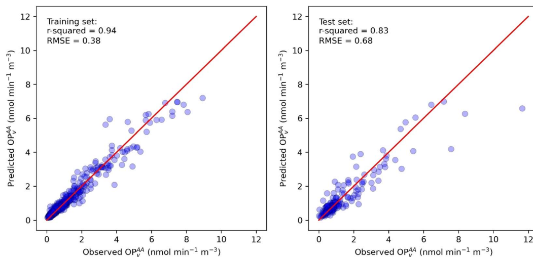
Fig. 3 Comparison between the observed and RF-predicted OP_{AA} ( \text{nmol min}^{-1} \text{m}^{-3} ) of PM_{10} for the training ( x samples) and testing ( y samples) sets in the GRE site. Note: red line represents the 1:1 line.
