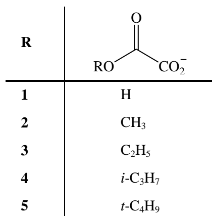
Scheme 1: Alkyloxalate ions investigated in this work.
