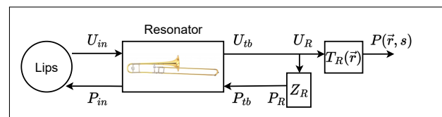
Figure 1. Description of the trombone, acoustic variables and conventions. The flow is counted positively when it occurs from the mouth to the bell.
