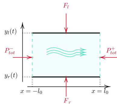
Figure 2. Glottal flow schematic, from [7].
