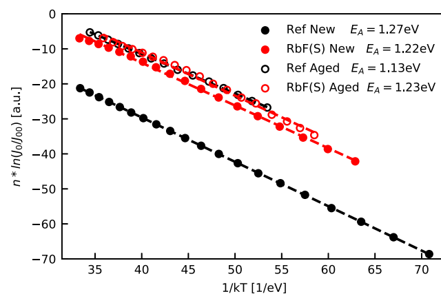
Figure 5. Arrhenius plot of n \cdot \ln(J_0/J_{00}) versus 1/kT with linear fits to the data. The activation energy is calculated from the slope of the fit (dashed lines).
