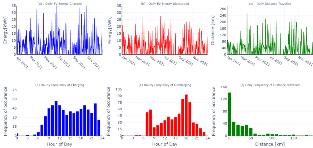
Figure 2: Daily usage summary of EV (a) Energy charged, (b) energy discharged, and (c) distance traveled and the distribution of EV (d) hourly count of vehicle charging, (hourly count of vehicle discharge, (f) frequency of distance traveled data – typical daily distance less than 50km
