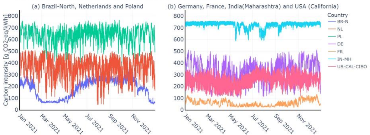
Figure 3: Hourly carbon intensity for the electricity grids of (a) Brazil-North, Netherlands, and Poland, and (b) Germany, France, India (Maharashtra), and USA (California)
