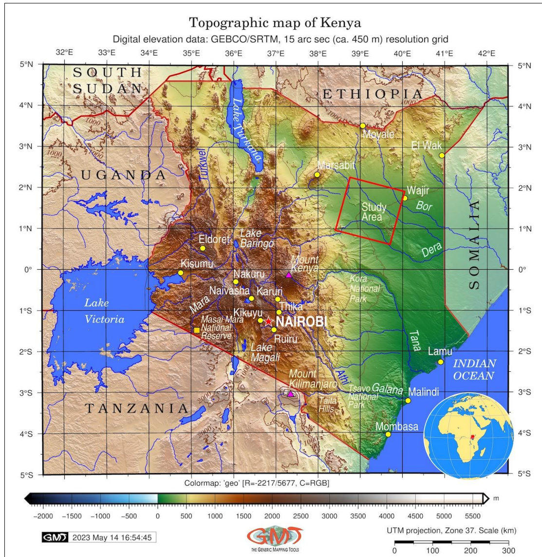
Figure 1: Topographic map of Kenya with study area (red rotated square). Data source: GEBCO. Mapping: GMT scripting toolset.
