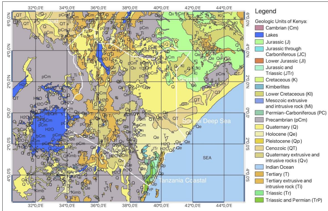
Figure 2: Geologic units, lithology and provinces in Kenya. Data source: geologic vector layers obtained from USGS.
