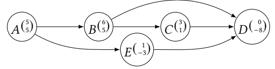
Figure 2. A schedule graph for the task graph of Fig. 1 in the PBC model.
