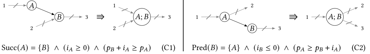
Figure 3. Clustering rules for single successor (left) and single predecessor (right). Striked through arrows \cancel{\rightarrow} represent 0 or more incoming/outgoing edges.
