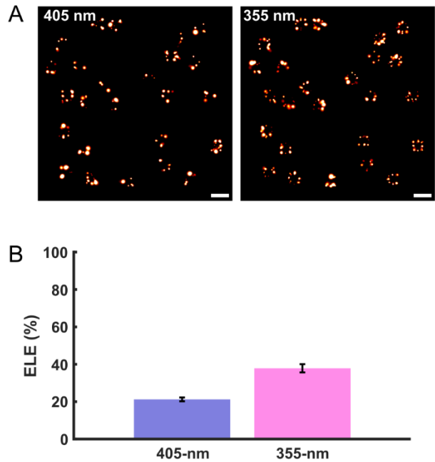
Figure 8. Simulated cryo-SMLM experiments of quantitative imaging of NPCs. (A) Reconstructed images using 355 nm or 405 nm illumination. (B) Effective Labeling Efficiency (ELE) using 355 nm or 405 nm illumination. ELE was extracted from the analysis of 100 NPCs (Fig. S19) and error bars were derived by bootstrapping. Scale bar: 0.5 \mu m.
