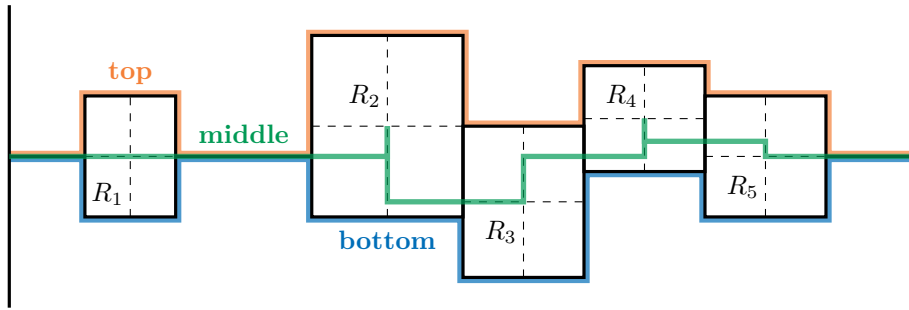
Figure 5: In orange, the top polyline of the s - t path formed by R_1, R_2, R_3, R_4 and R_5 . In blue, its bottom polyline, and in green, its middle polyline. The dashed lines split their respective rectangles into 4 equal parts.
