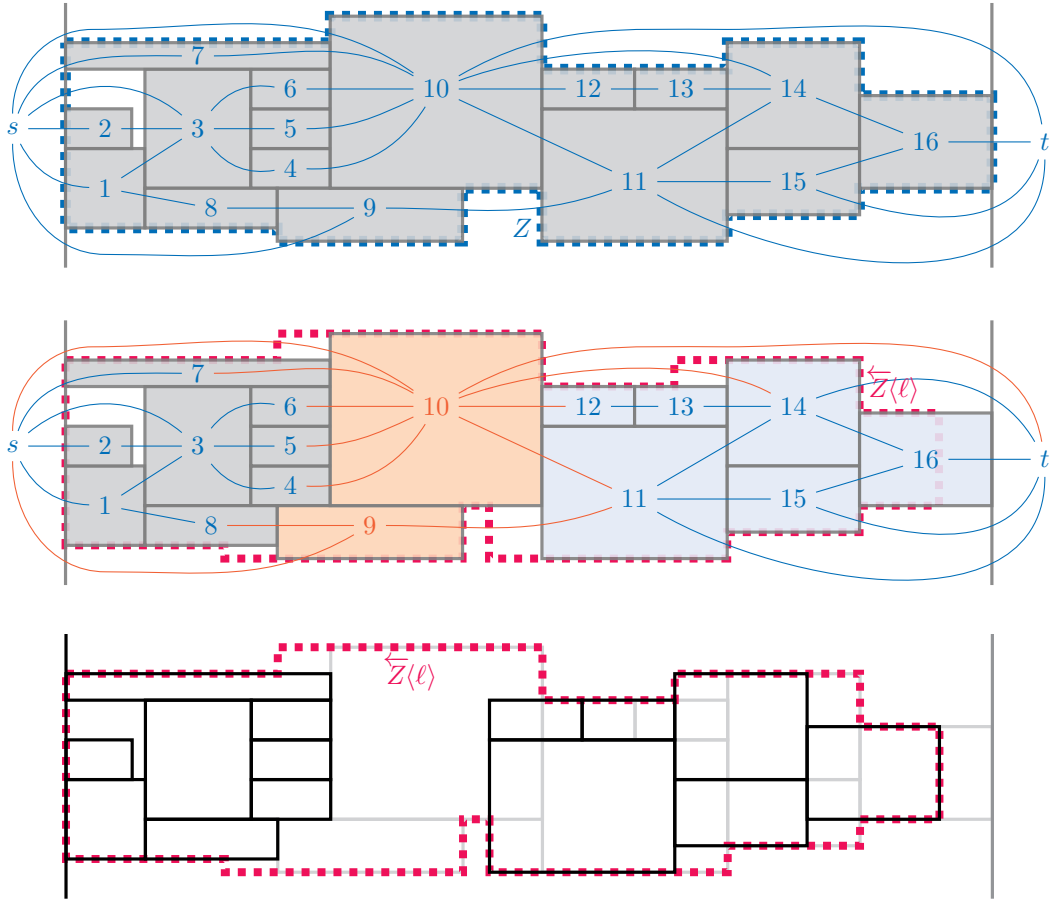
Figure 3: Illustration of the proof of Proposition 15. From top to bottom: First, a blue conflict graph of the gray packing. The packing is entirely in Z , delimited by the blue border. Secondly, we remove the orange separator C and want to pack the leftover rectangles inside the red region \overleftarrow{Z}(\ell) . The set of rectangles referred to as Y in the proof is in light blue, and X is left gray. Finally, we pack in \overleftarrow{Z}(\ell) by shifting the rectangles at the right of the separator by \ell to the left.
