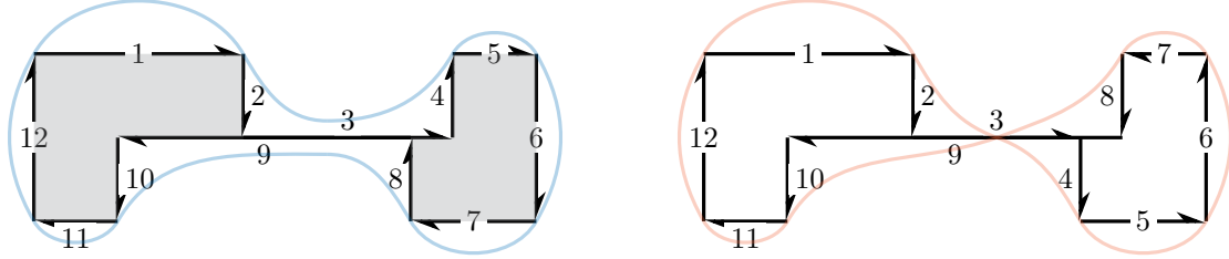
Figure 1: Left panel: an example of a container where the order of the segments is given by the numbers, and some injective candidate \gamma_\varepsilon in light blue. Right panel: an example of a non-container (the paths cross in the middle), and some candidate \gamma_\varepsilon in light red, that is not injective.
