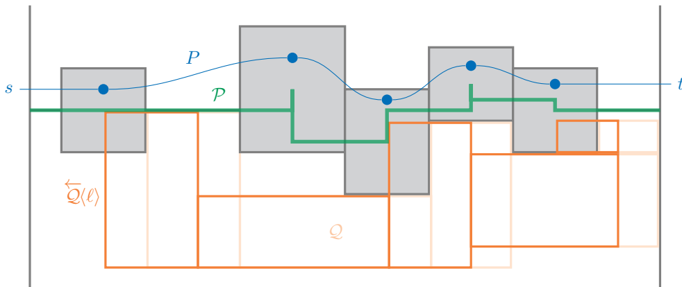
Figure 6: In green, the middle polyline \mathcal{P} of the blue s - t path P constituted of the gray rectangles. In light orange, \mathcal{Q} , and in orange, \overline{\mathcal{Q}}(\ell) . Notice that the green polyline does not cross any orange rectangles.
