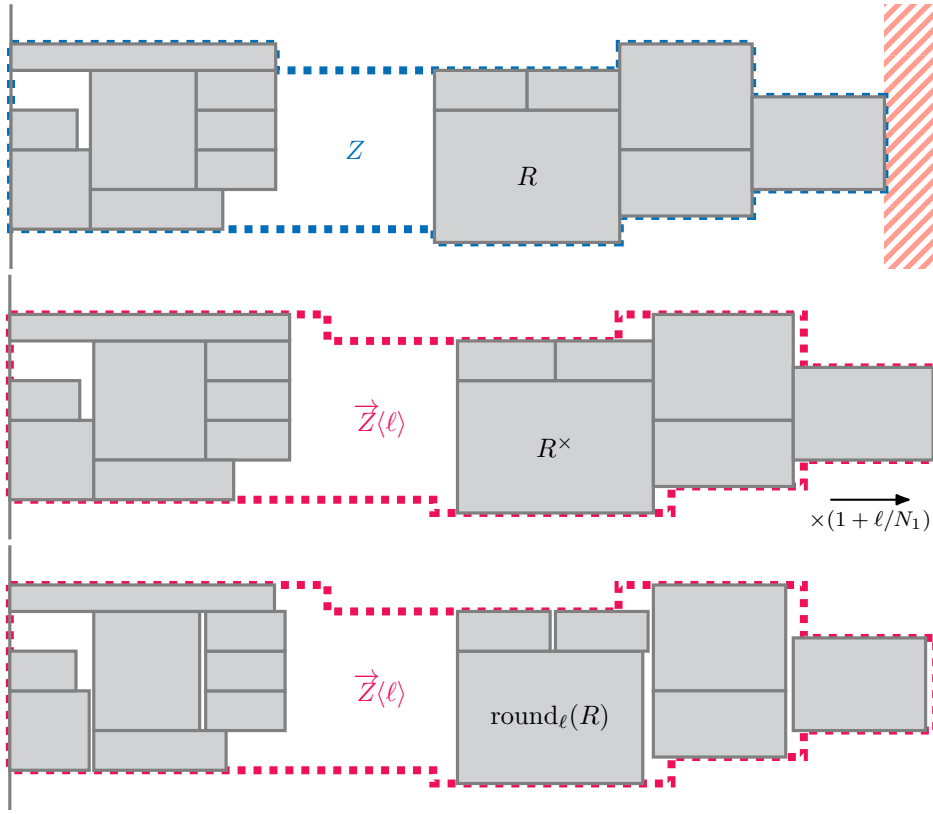
Figure 4: Illustration of the proof of Proposition 16. From top to bottom: First, \mathcal{Q} is packed into Z (blue zone). Then, the rectangles in \mathcal{Q} are scaled horizontally by a factor \lambda = 1 + \ell/N_1 . We argue in the proof that these scaled-up rectangles are packed in \vec{Z}(\ell) (red zone). Finally, we replace each scaled-up rectangle by its rounded version, which has smaller width.
