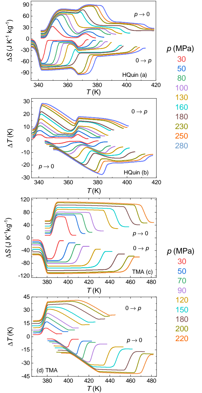
Fig. 8 Barocaloric effects obtained on first application or removal of pressure. Isothermal entropy changes on decompression and compression as a function of temperature at different pressures for HQuin (a) and TMA (c). Adiabatic temperature changes on decompression and compression as a function of temperature at different pressures for HQuin (b) and TMA (d).
