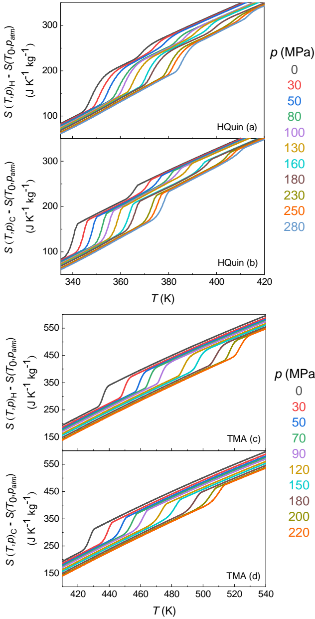
Fig. 7 Temperature-dependent isobaric entropy curves at different pressures, both upon heating (a,c), and cooling (b,d) for HQuin and TMA.
