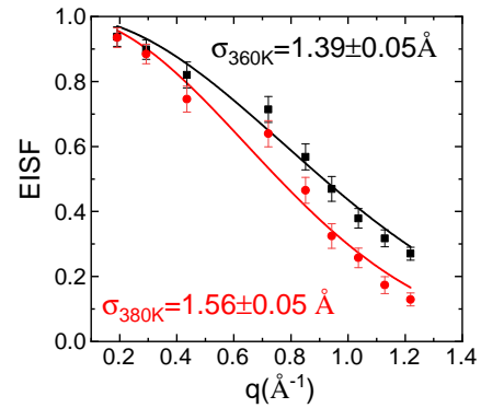
Fig. 4 Elastic Incoherent Structure Factor obtained for HQuin as a function of momentum transfer for the two measured temperatures ( T = 380 K red circles, T = 360 K black squares). Solid lines are fits of the experimental data to equation 2.
