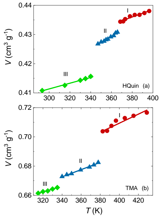
Fig. 5 Temperature-dependent unit cell volume on heating for HQuin (a) and TMA (b). Error bars are smaller than the symbol size. The lines are linear fits to V(T) data.
