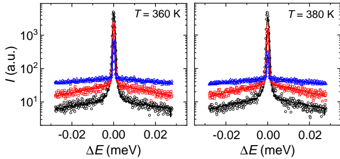
Fig. 3 Representative experimental neutron scattering spectra of HQuin for selected momentum transfer (symbols) ( q_1 = 0.29 Å: black circles, q_2 = 0.85 Å: red squares, q_3 = 1.22 Å: blue triangles). The spectrum at momentum transfer q_3 has been shifted upwards by 20 units. Lines show the fittings using equation 1.
