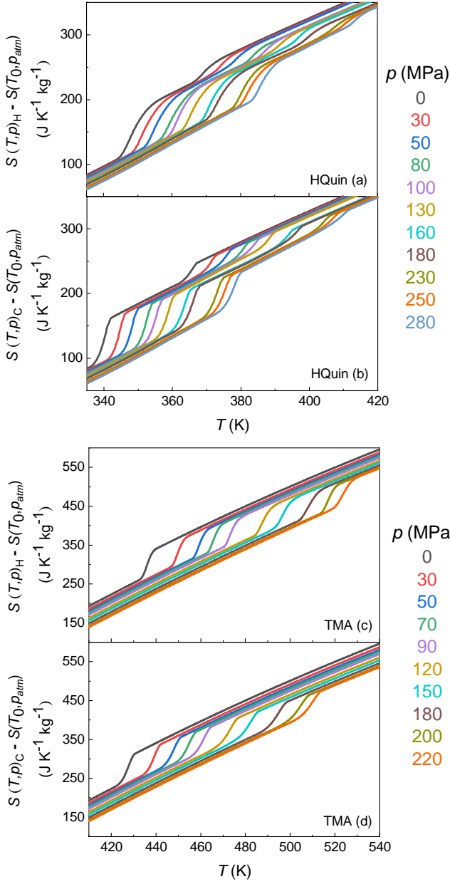
Fig. 7 Temperature-dependent isobaric entropy curves at different pressures, both upon heating (a,c), and cooling (b,d) for HQin and TMA.
