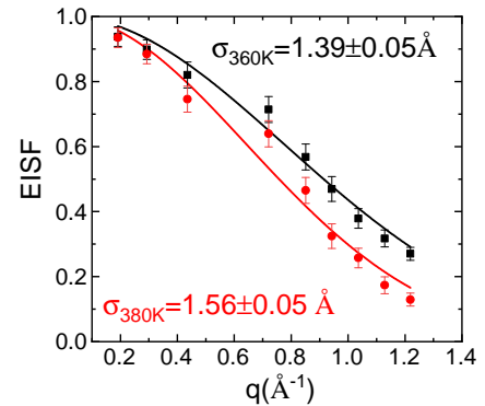
Fig. 4 Elastic Incoherent Structure Factor obtained for HQuin as a function of momentum transfer for the two measured temperatures ( T = 380 K red circles, T = 360 K black squares). Solid lines are fits of the experimental data to equation 2.
