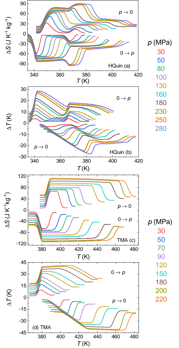
Fig. 8 Barocaloric effects obtained on first application or removal of pressure. Isothermal entropy changes on decompression and compression as a function of temperature at different pressures for HQin (a) and TMA (c). Adiabatic temperature changes on decompression and compression as a function of temperature at different pressures for HQin (b) and TMA (d).
